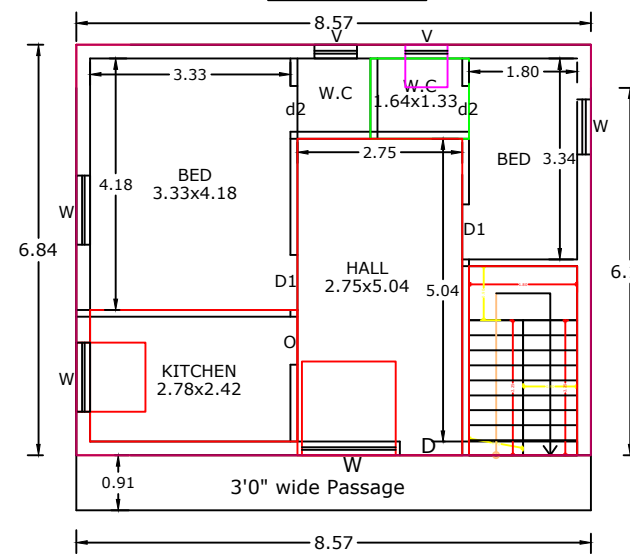
EXISTING APPROVED GROUND FLOOR PLAN
