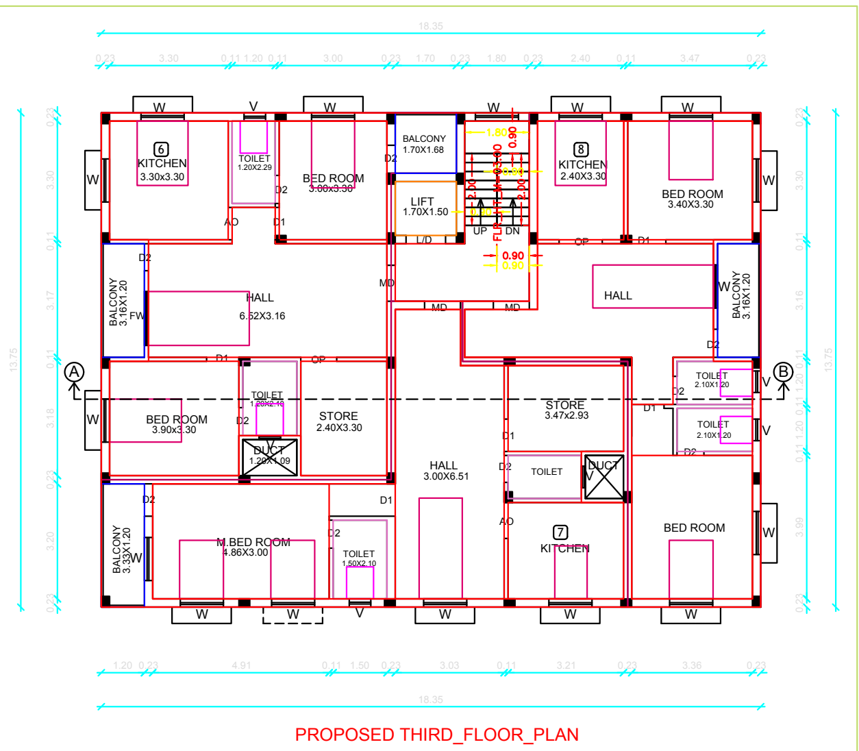
PROPOSED THIRD FLOOR PLAN THIRD FLOOR PLAN (PROPOSED)
