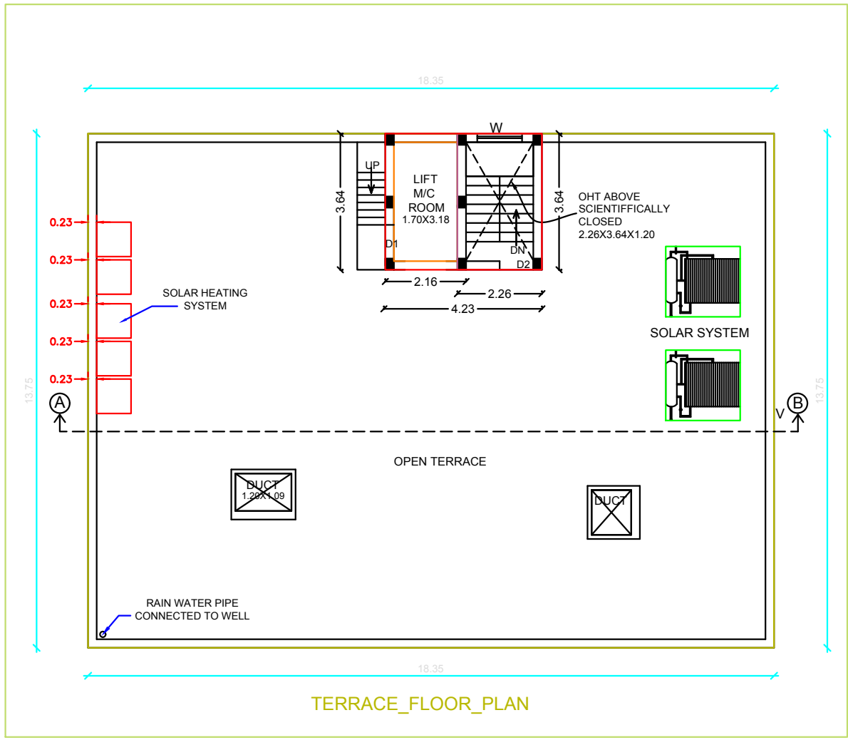
TERRACE FLOOR PLAN (PROPOSED)
