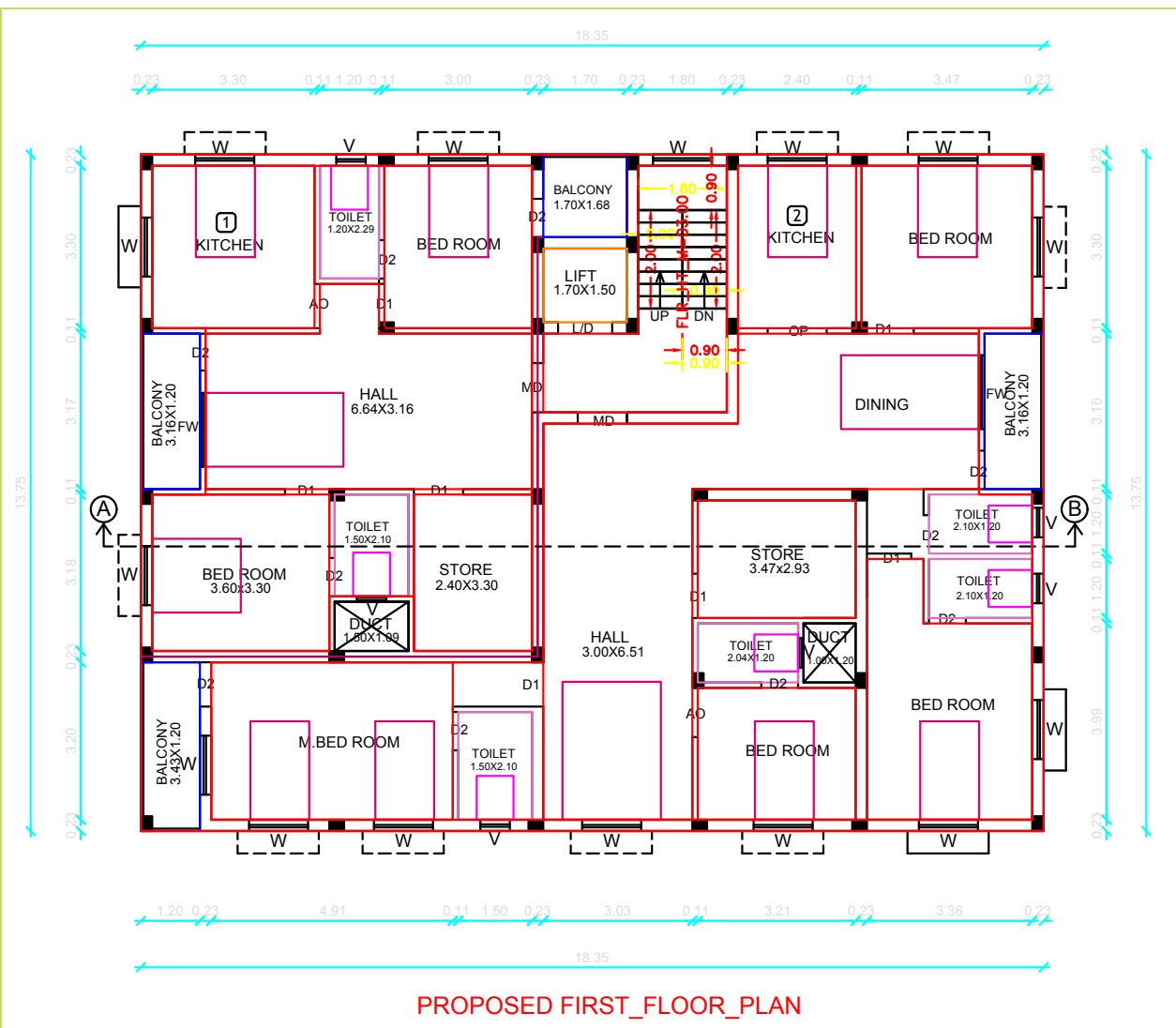
PROPOSED FIRST FLOOR PLAN FIRST FLOOR PLAN (PROPOSED)
