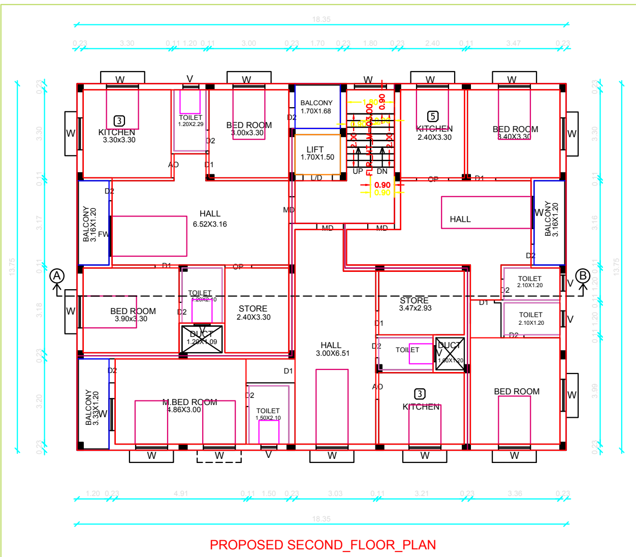
PROPOSED SECOND FLOOR PLAN SECOND FLOOR PLAN (PROPOSED)
