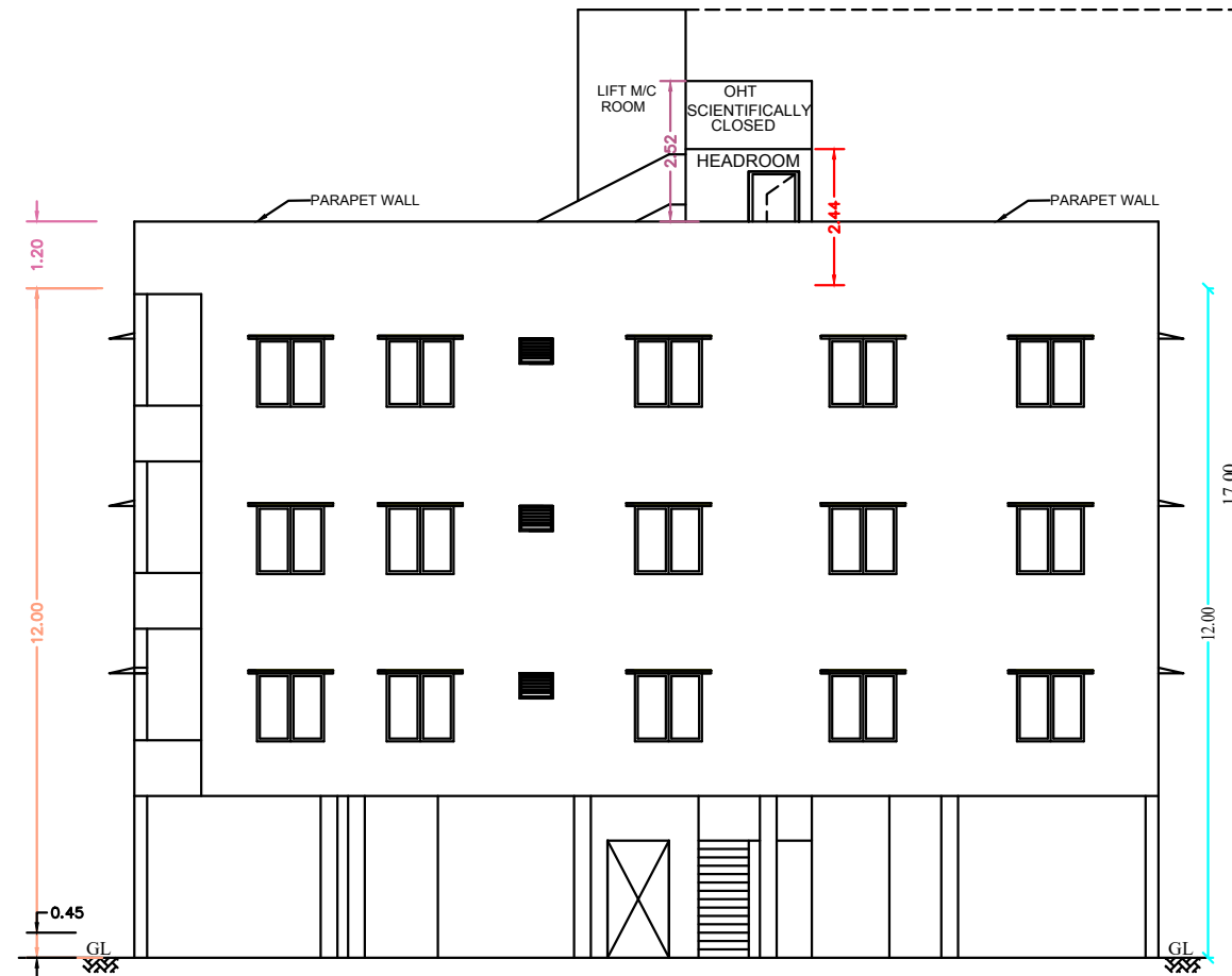
FRONT ELEVATION
