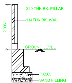
SECTION OF GATE
