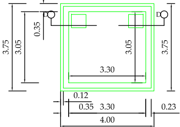
PLAN (CAPACITY: 21500 LITERS) DETAILS OF RAIN WATER COLLECTION SUMP
