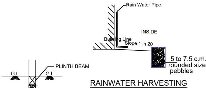
RAINWATER HARVESTING
