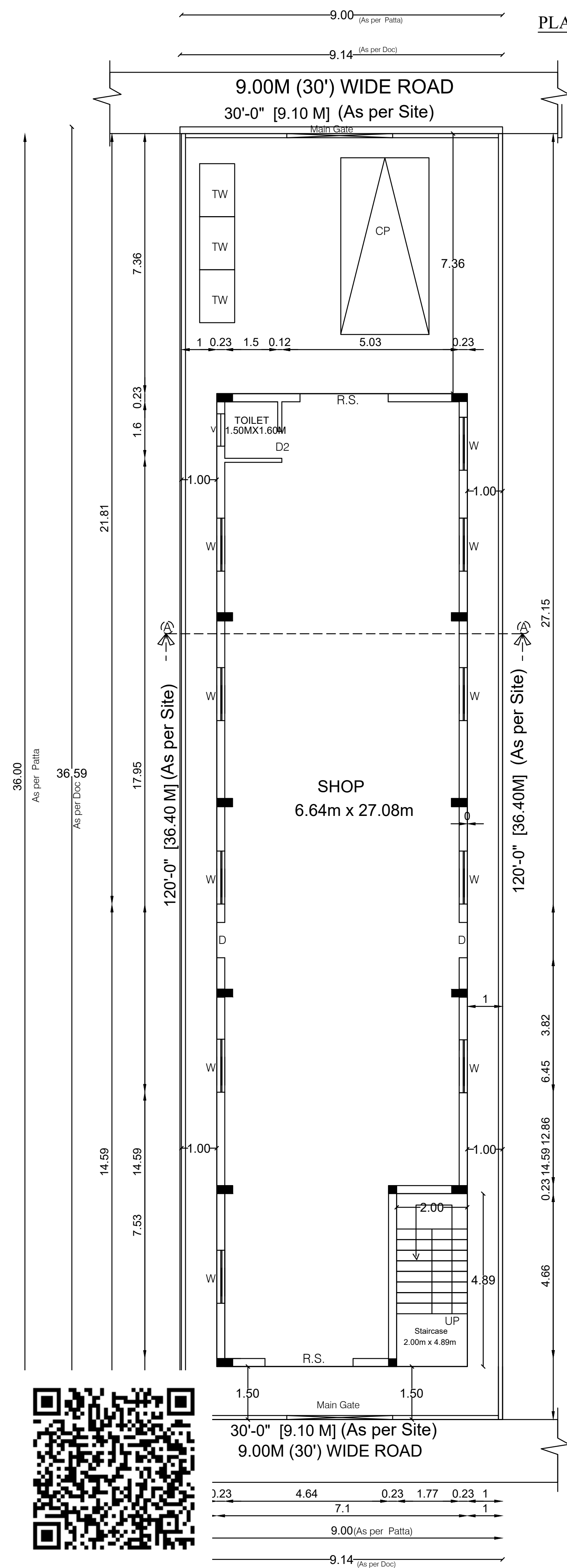
SITE CUM GROUND FLOOR PLAN (Proposed)
