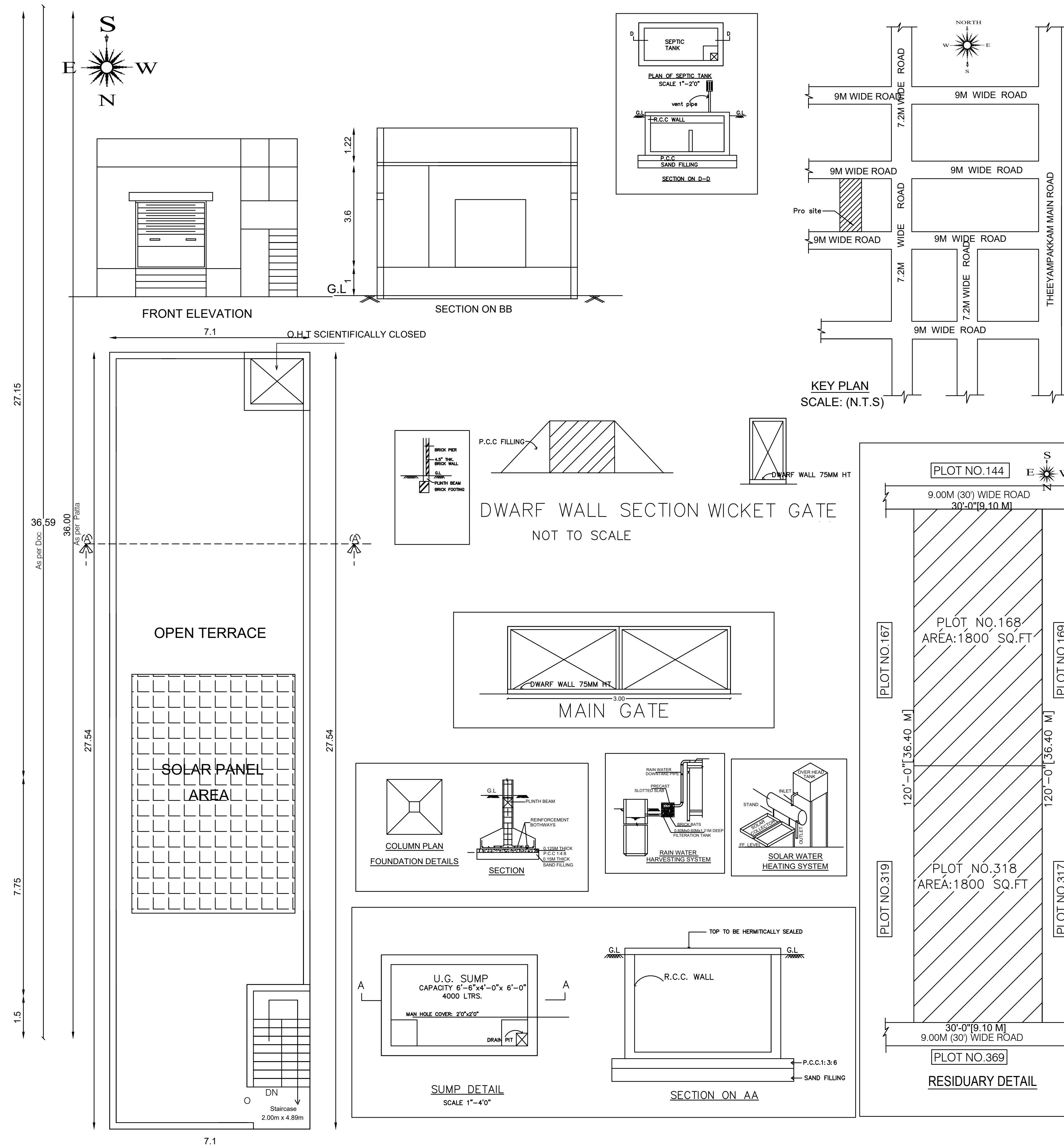
TERRACE FLOOR PLAN (Proposed)
