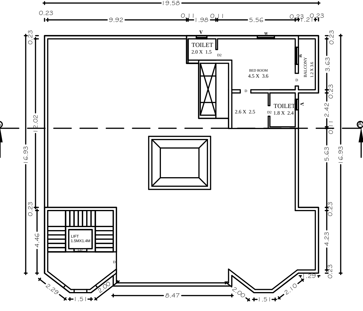
PARTLY SECOND FLOOR PLAN (PROPOSED)
