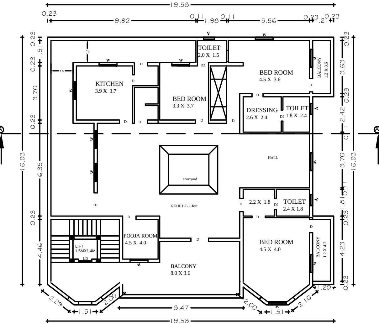
PARTLY FIRST FLOOR PLAN (PROPOSED)
