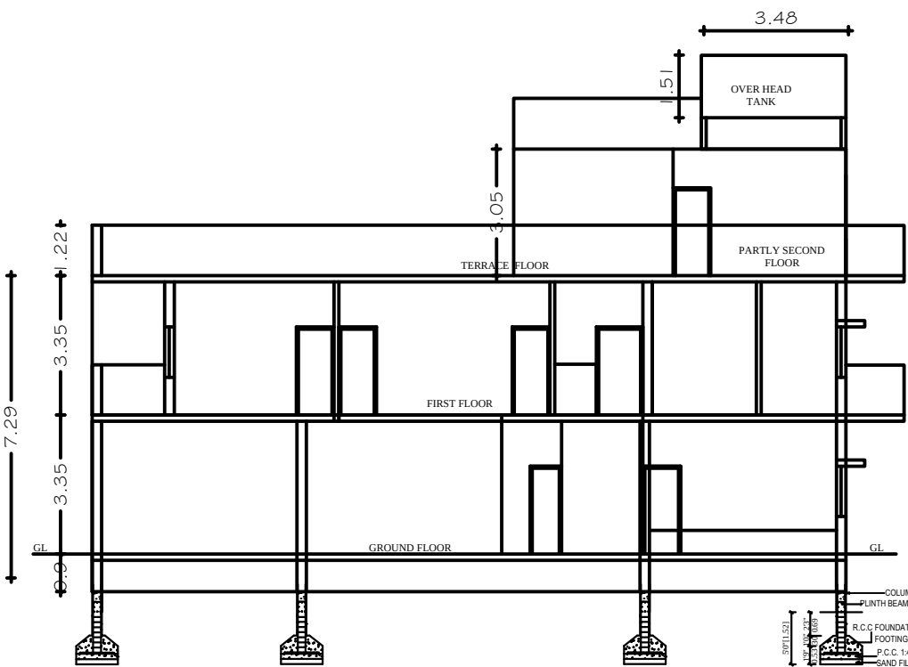
SECTION
