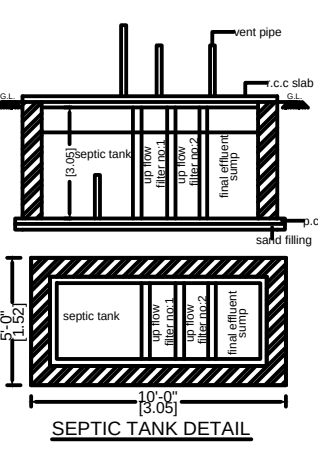
SEPTIC TANK DETAIL
