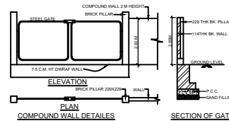
COMPOUND WALL DETAILS
