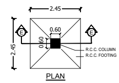
DETAILS OF COLUMN FOOTING
