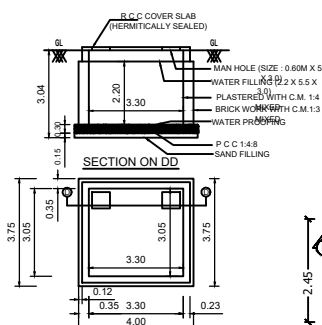
DETAILS OF RAIN WATER COLLECTION SUMP
