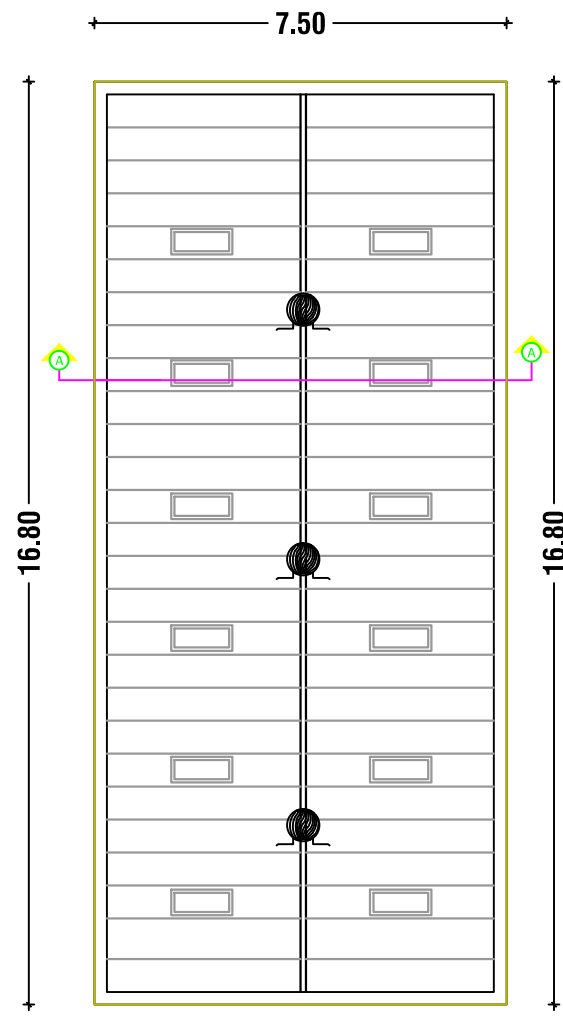
ROOF FLOOR PLAN (PROPOSED)
