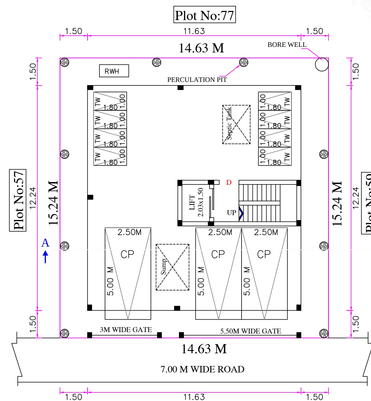
SITE CUM STILT FLOOR PLAN [ PROPOSED ]
