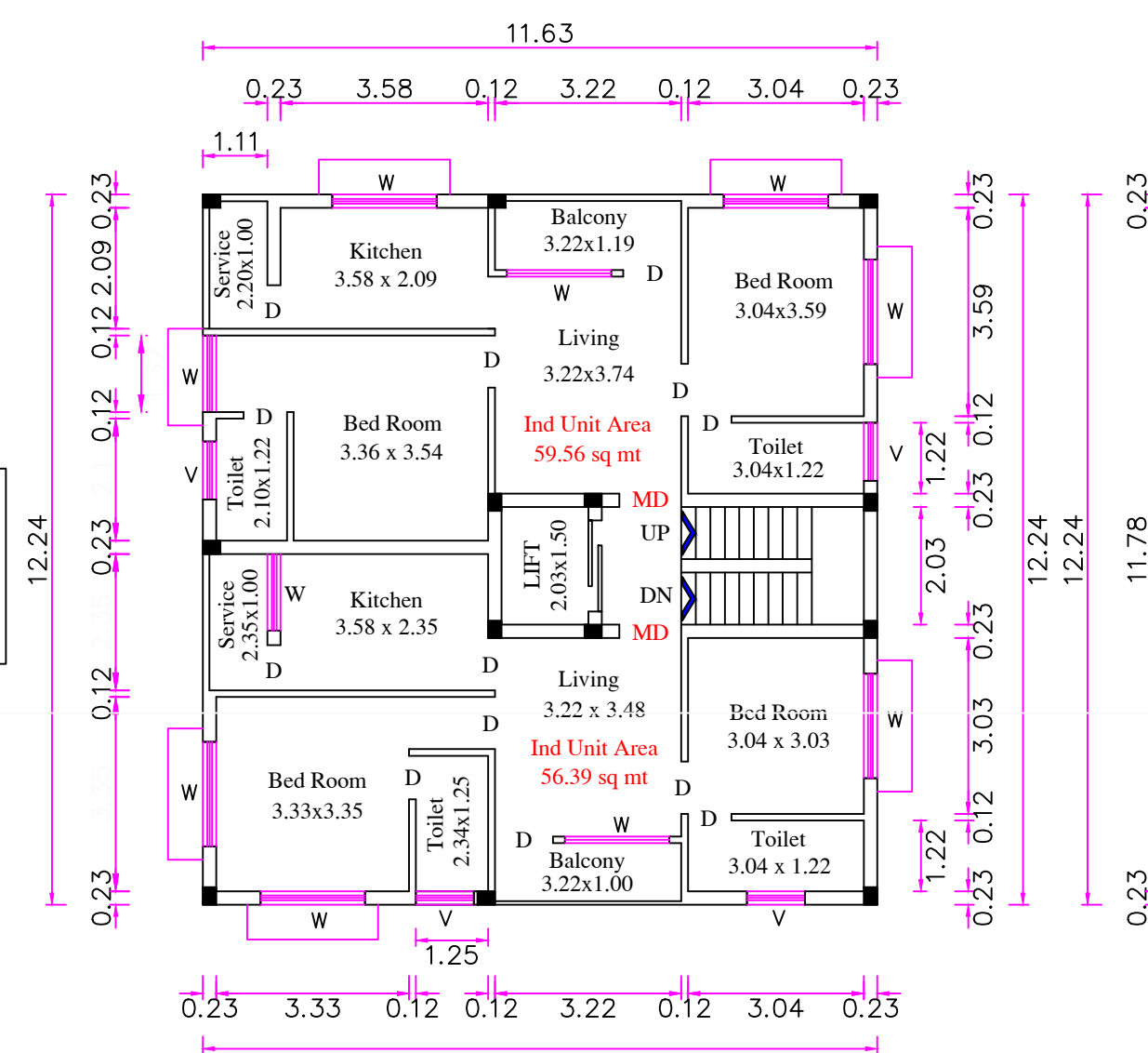
TYPICAL FLOOR PLAN [ FIRST , SECOND & THIRD ] [ PROPOSED ]
