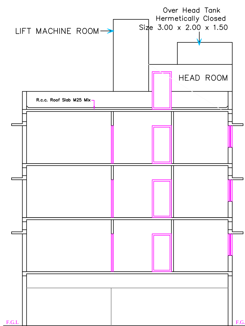
SECTION ON A - A PROPOSED
