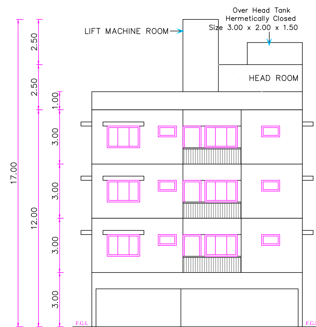
ELEVATION [ PROPOSED ]
