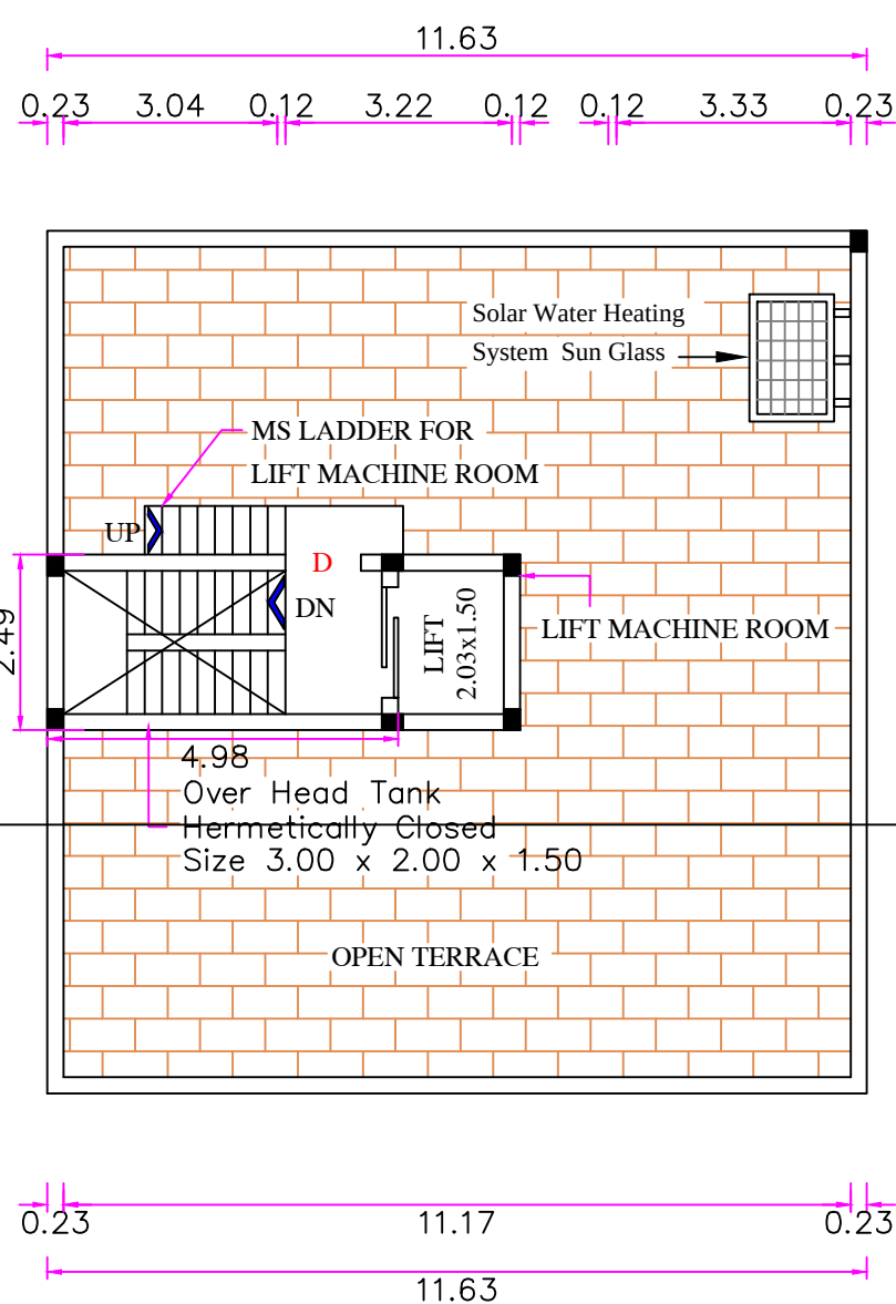
TYPICAL FLOOR PLAN [ PROPOSED ]
