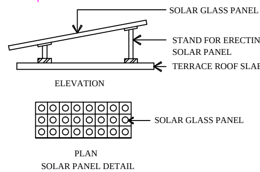
PLAN SOLAR PANEL DETAIL
