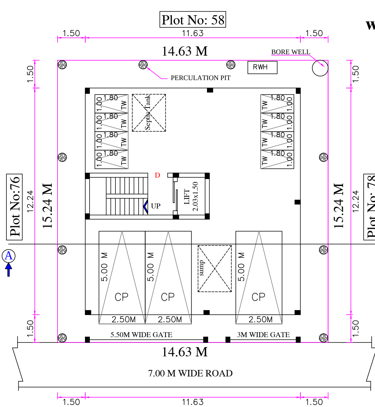
SITE CUM STILT FLOOR PLAN [ PROPOSED ]
