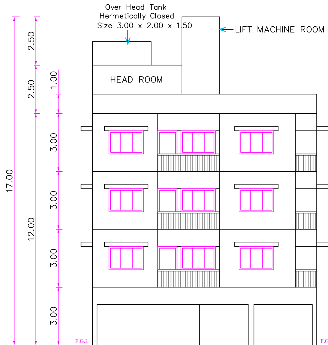
ELEVATION [ PROPOSED ]
