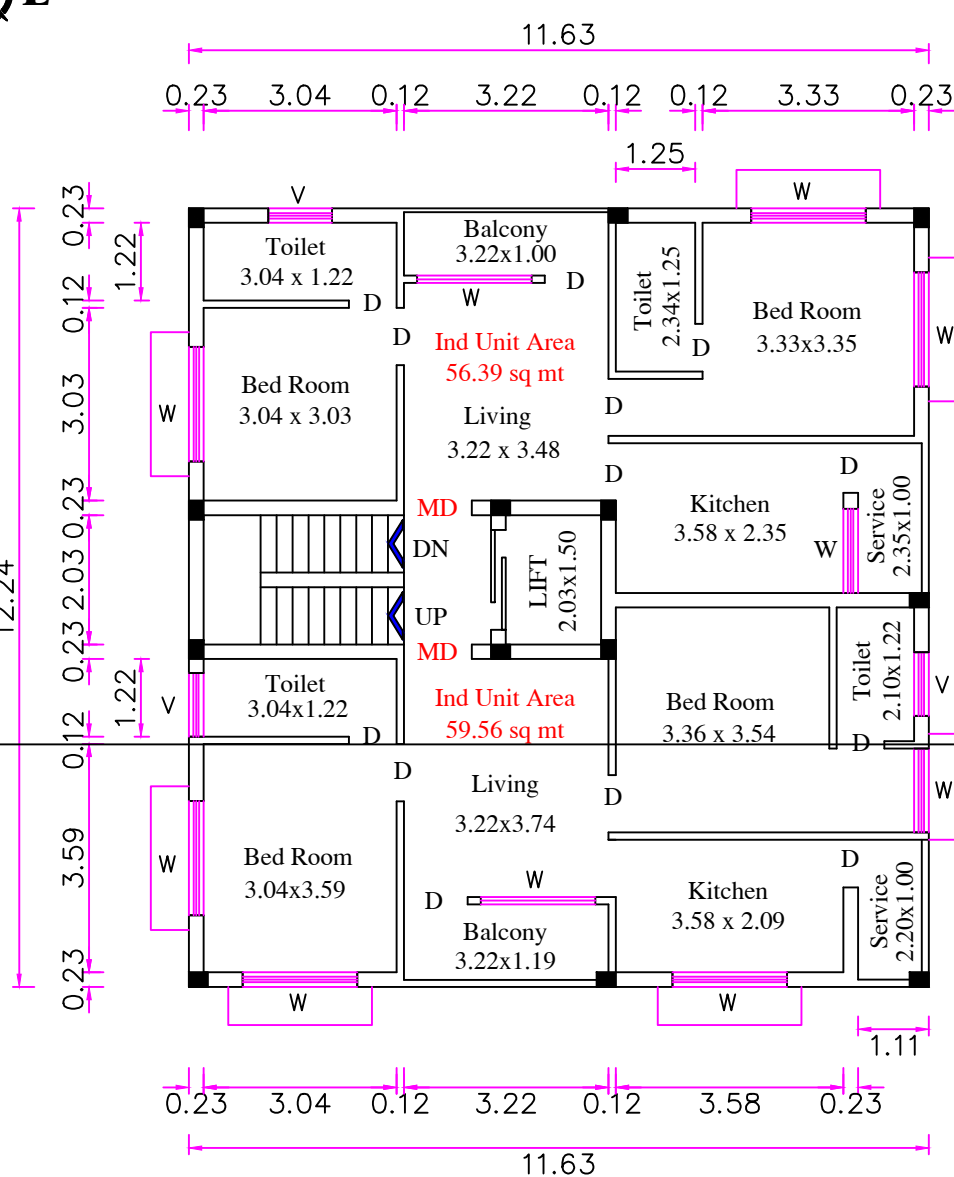
TYPICAL FLOOR PLAN [ FIRST , SECOND & THIRD ] [ PROPOSED ]
