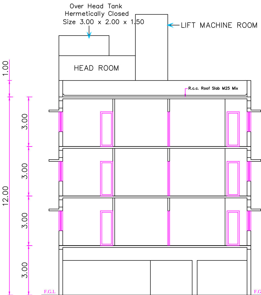
SECTION ON A - A PROPOSED
