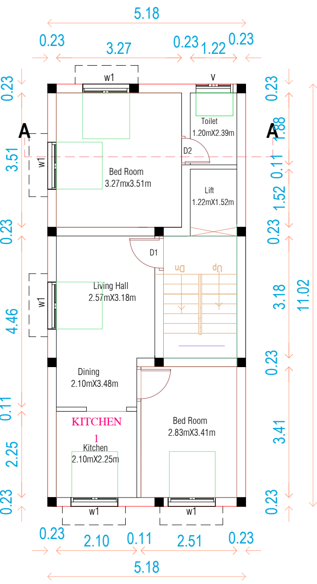
TYPICAL FIRST, SECOND, THIRD FLOOR PLAN
