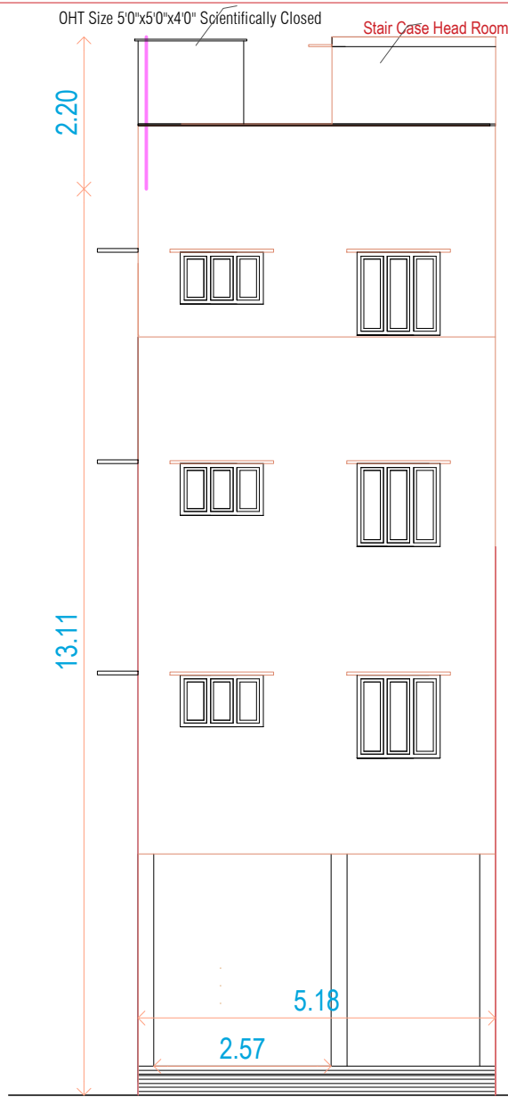
FRONT ELEVATION
