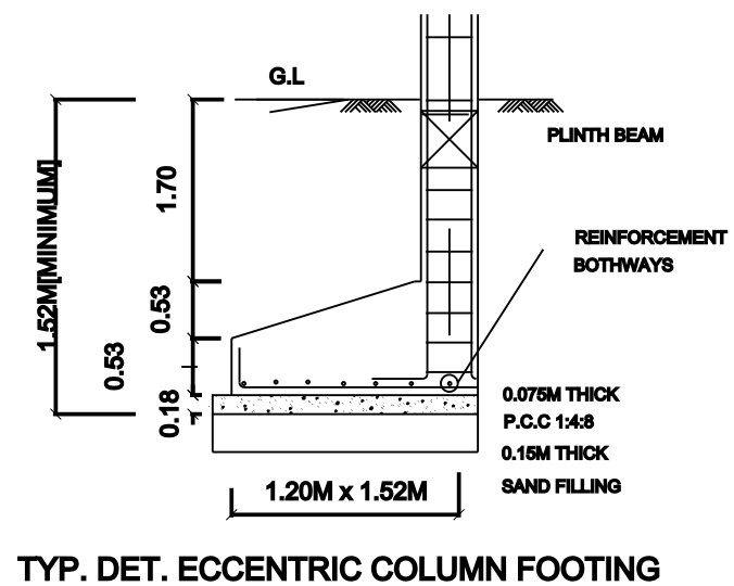
TYP. DET. ECCENTRIC COLUMN FOOTING
