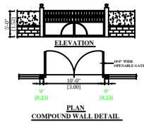
PLAN COMPOUND WALL DETAIL
