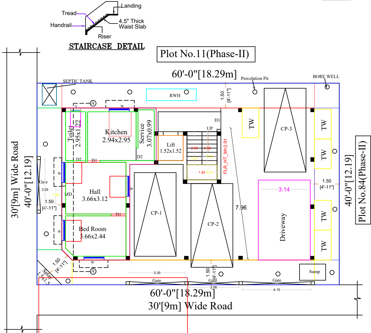
SITE CUM STILT AND GROUND FLOOR PART
