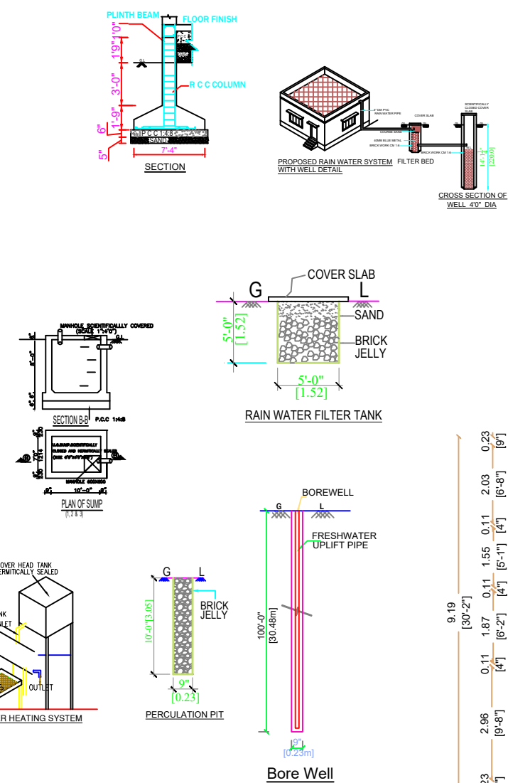
Bore Well
