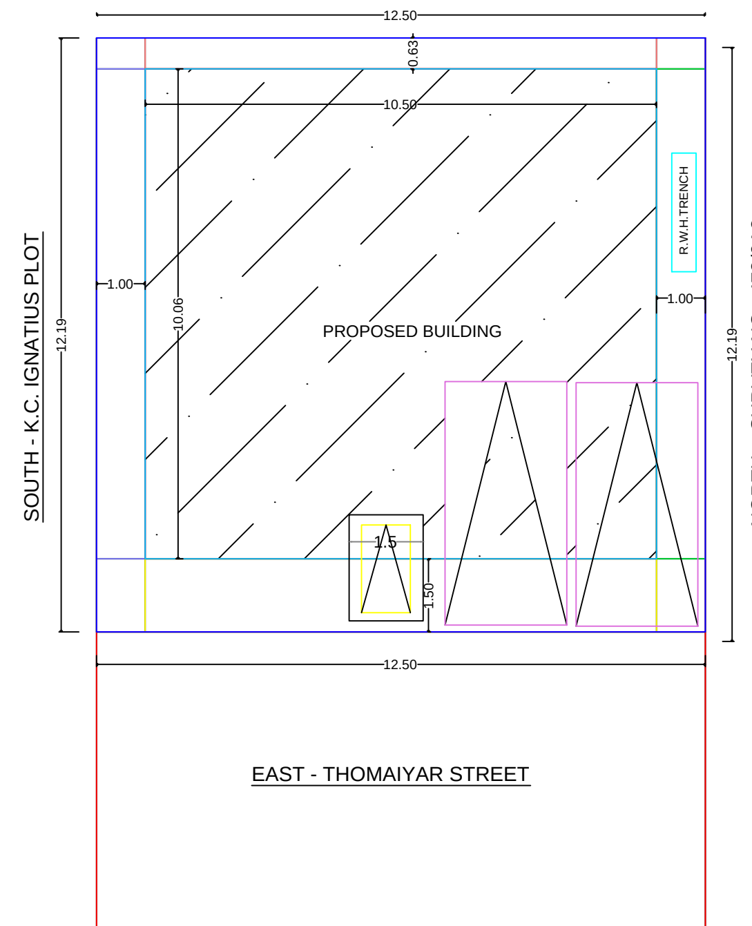
SITE PLAN
