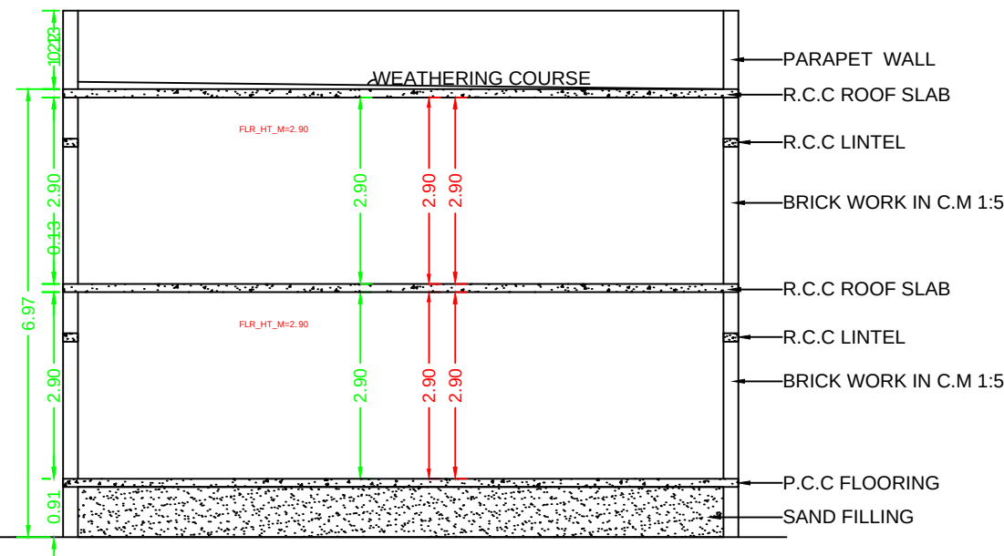
SECTION
