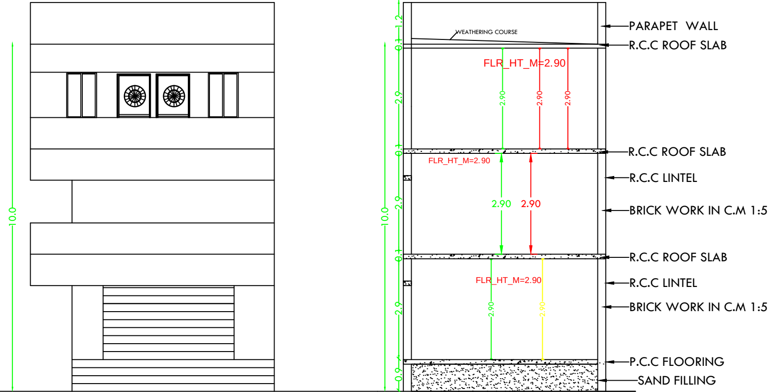
SECTION
