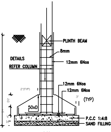
FOUNDATION DETAILS
