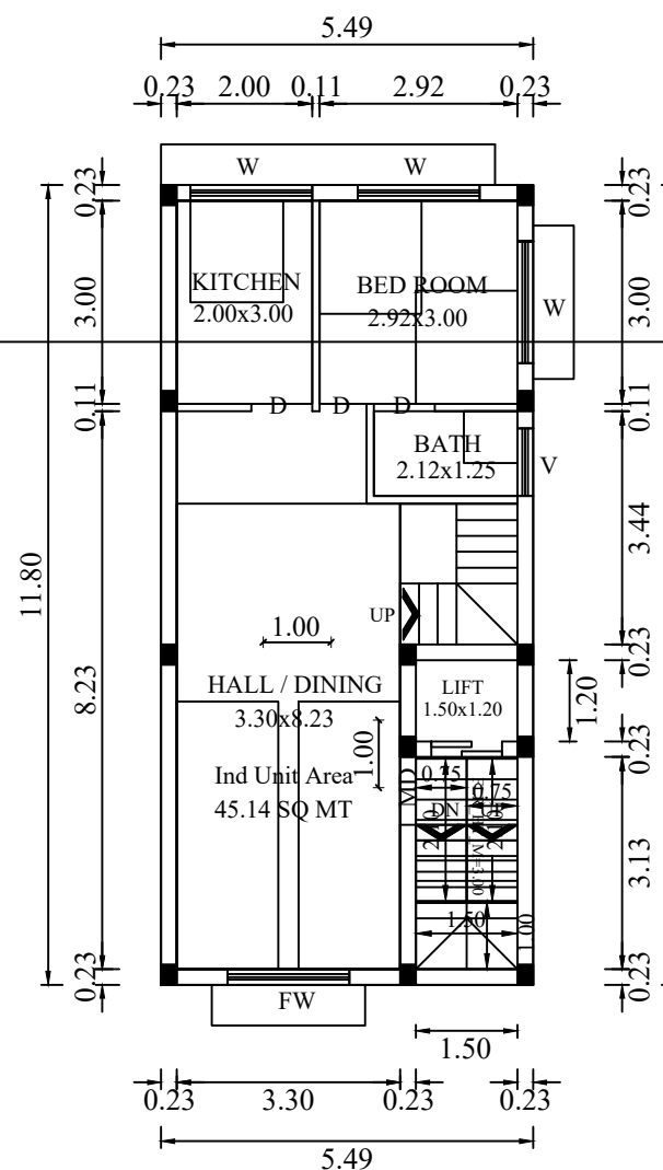
SECOND FLOOR PLAN [ PROPOSED ]
