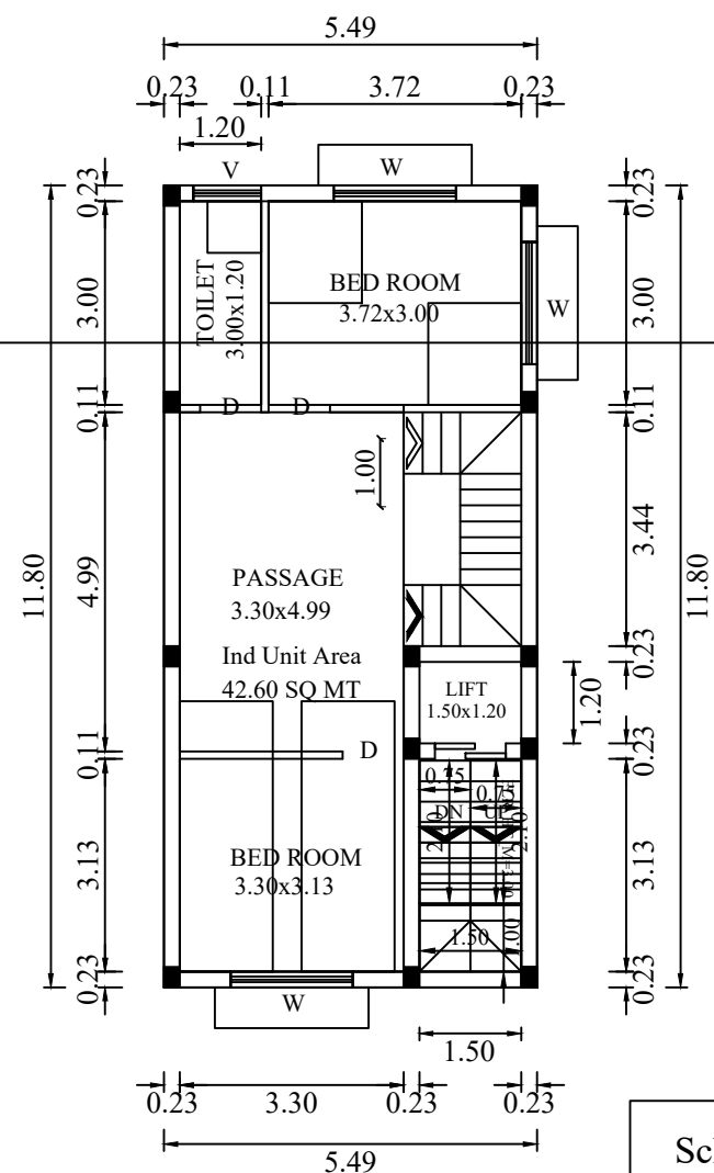
THIRD FLOOR PLAN [ PROPOSED ]
