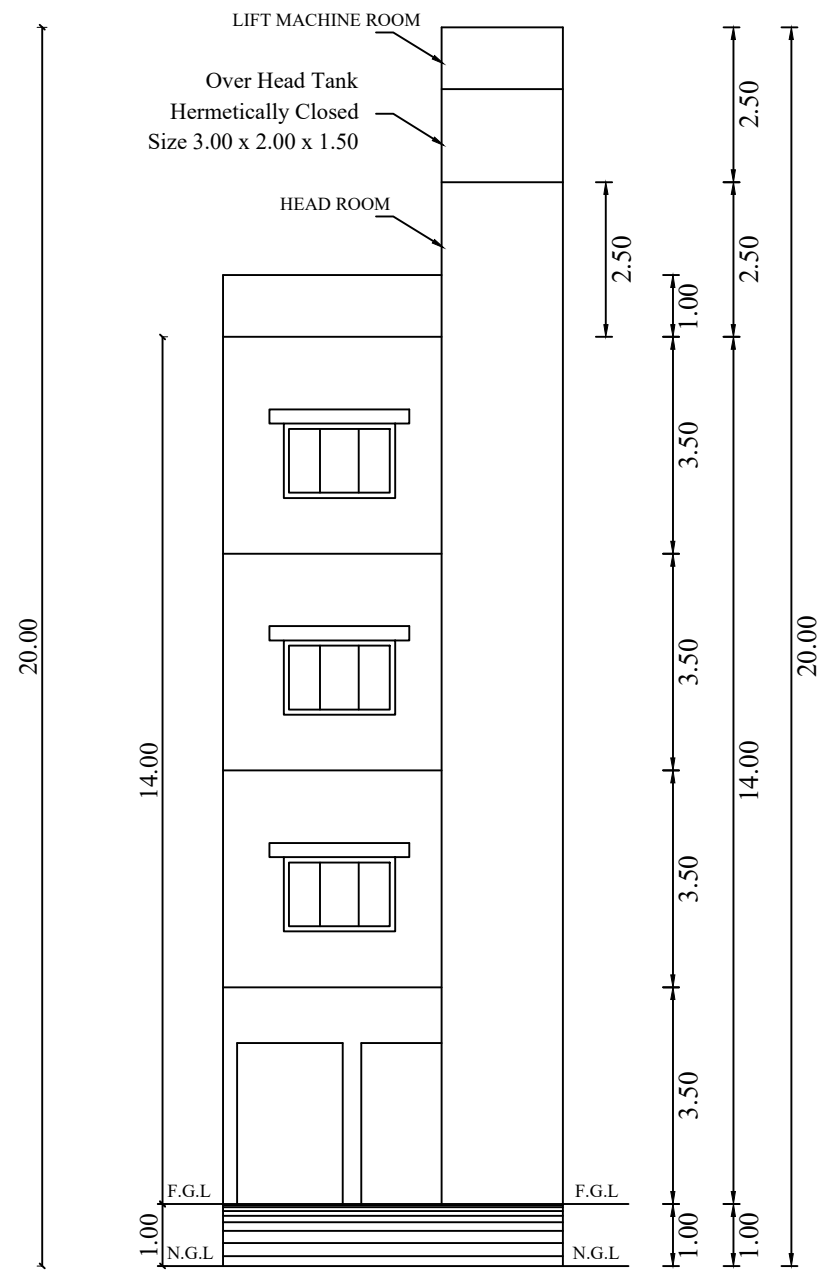
ELEVATION PROPOSED
