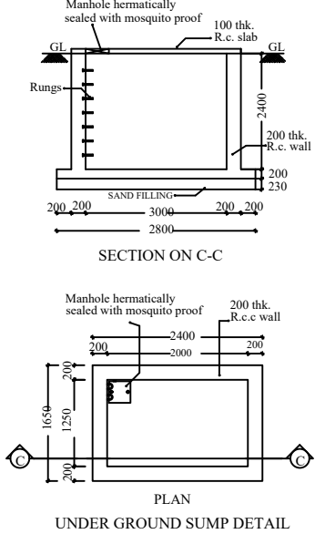
UNDER GROUND SUMP DETAIL
