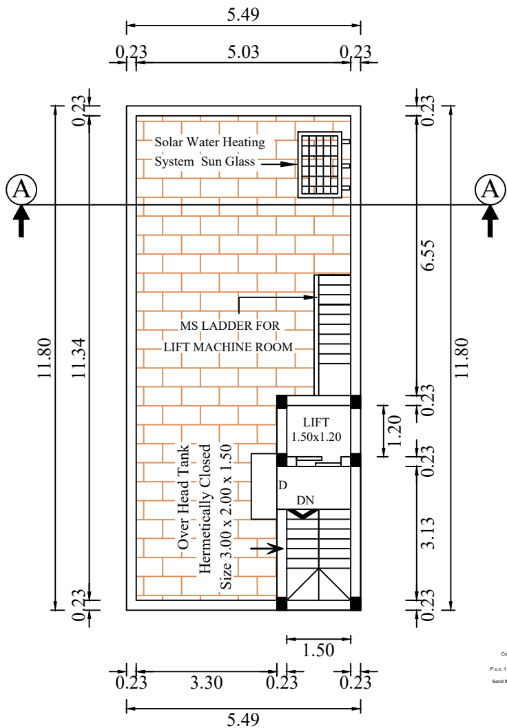
TERACE FLOOR PLAN [ PROPOSED ]
