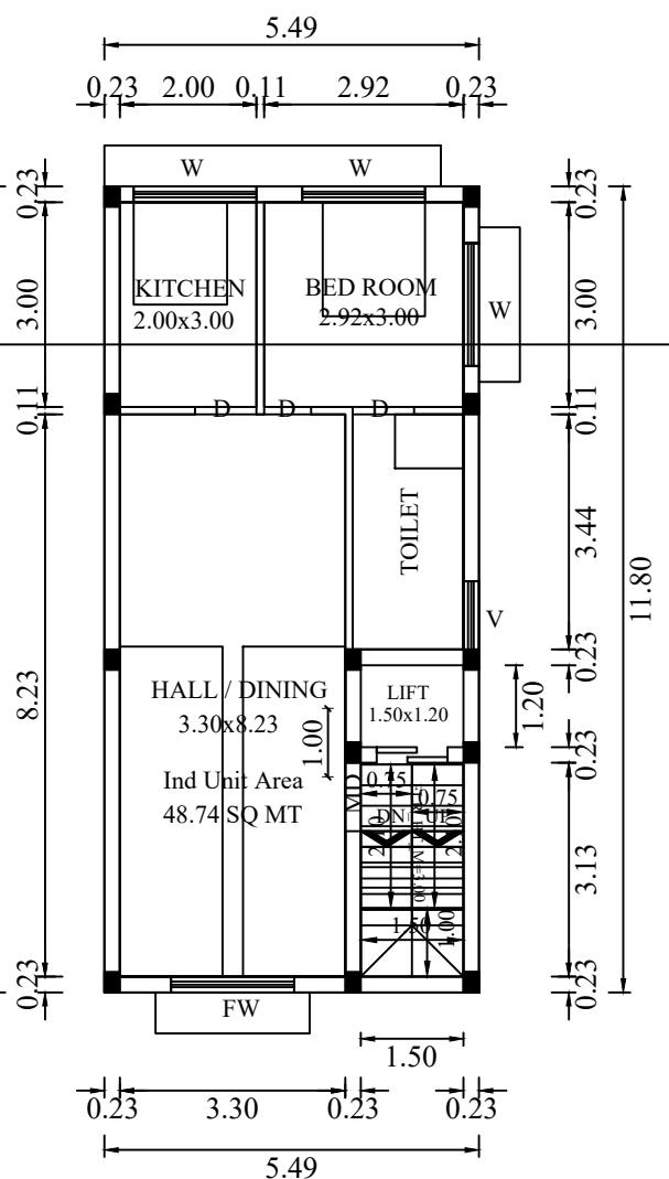
FIRST FLOOR PLAN [ PROPOSED ]
