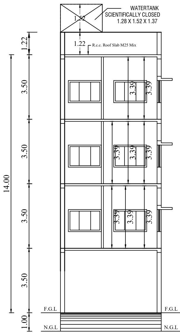
SECTION ON A - A PROPOSED
