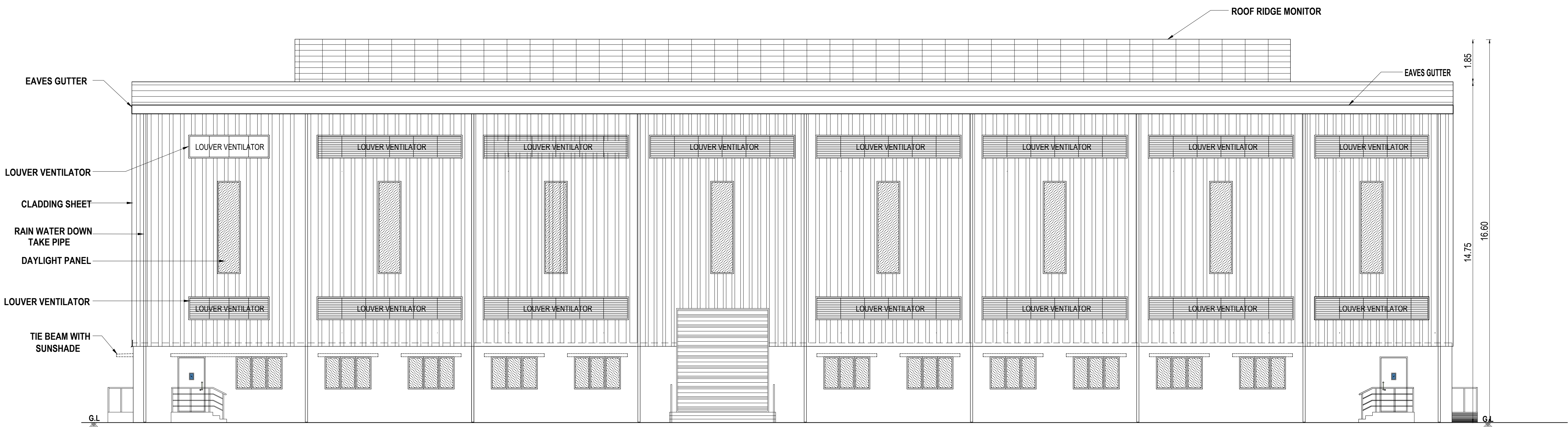
SOUTH FACE ELEVATION
