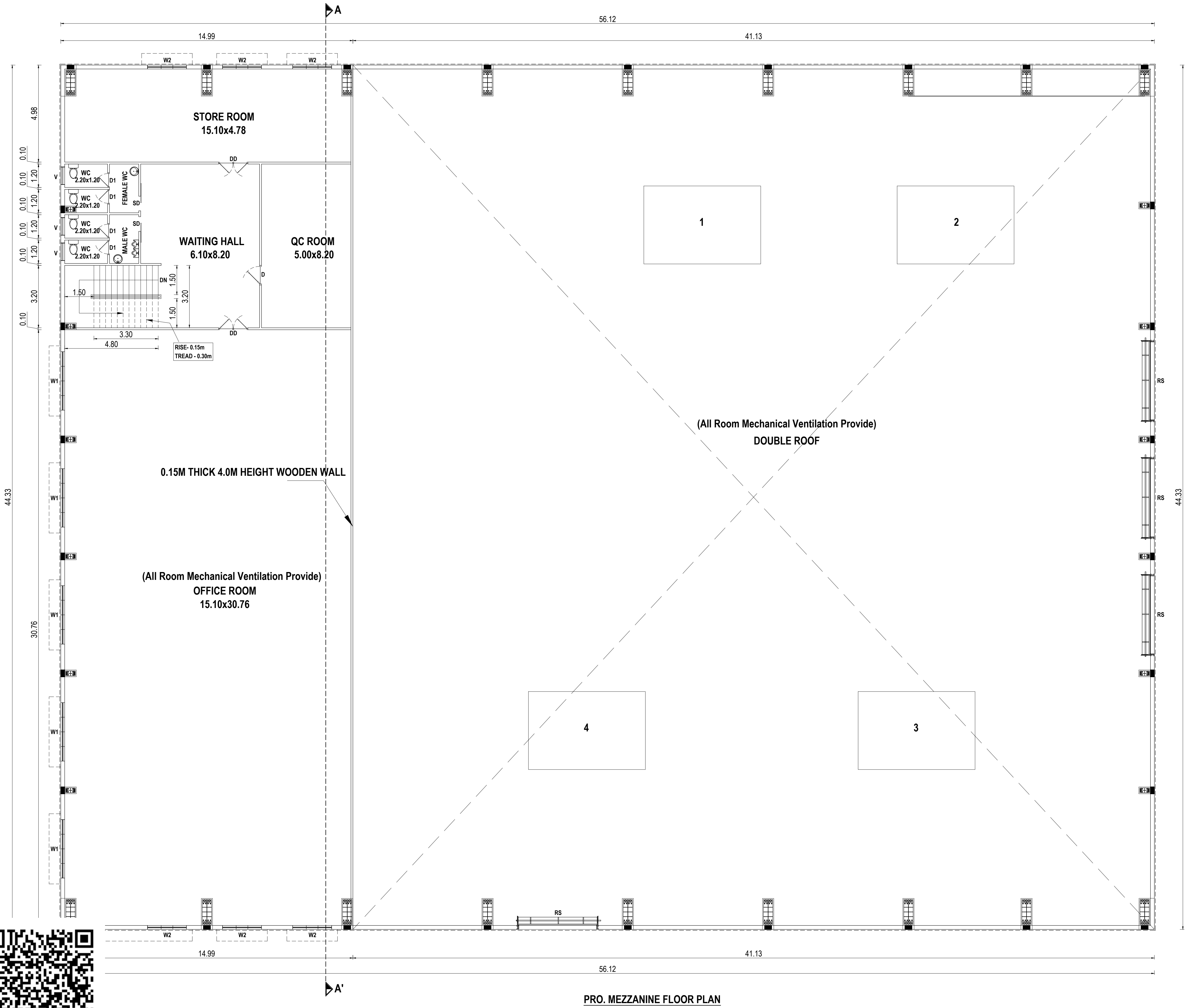
PRO. MEZZANINE FLOOR PLAN
