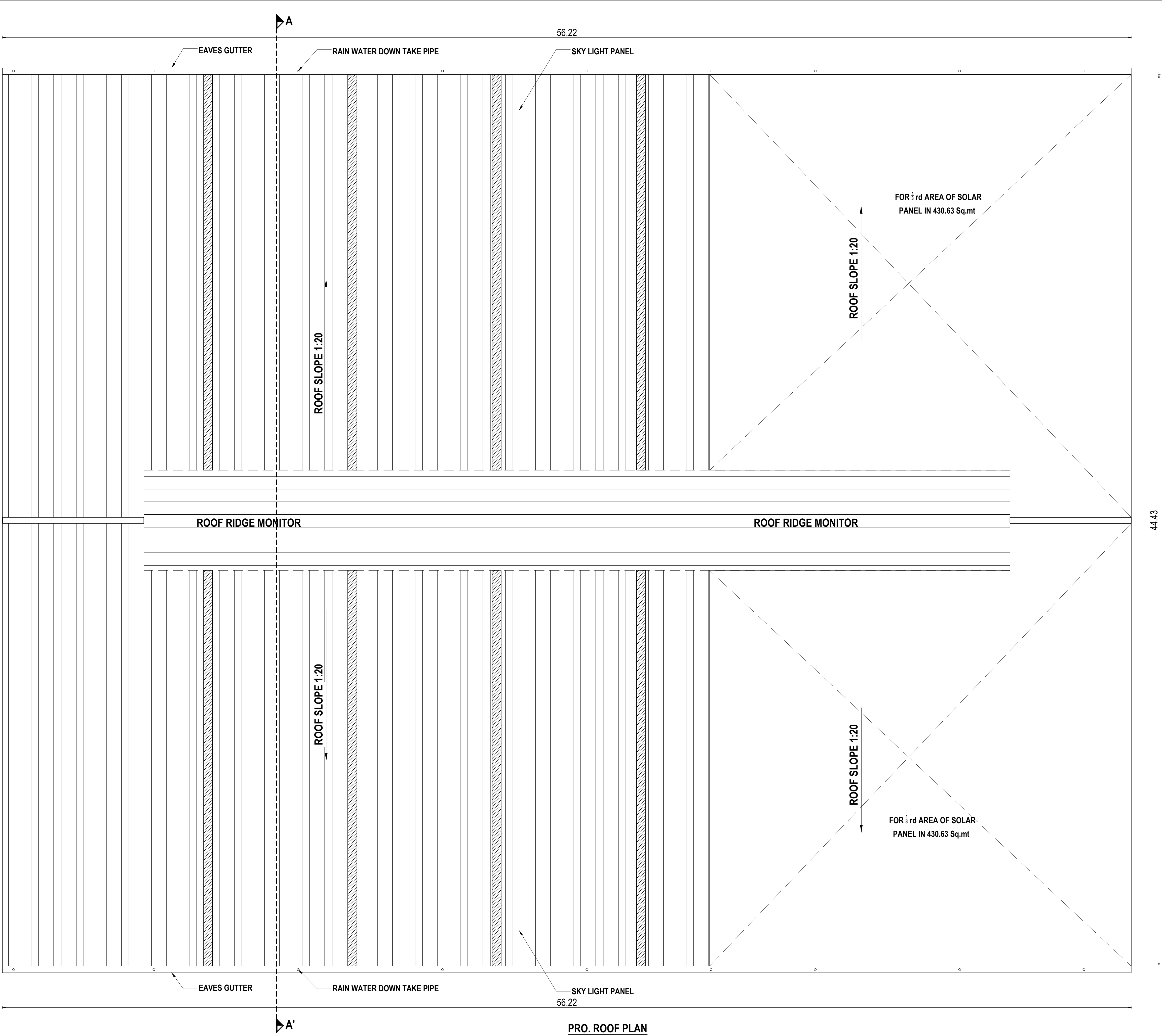
PRO. ROOF PLAN
