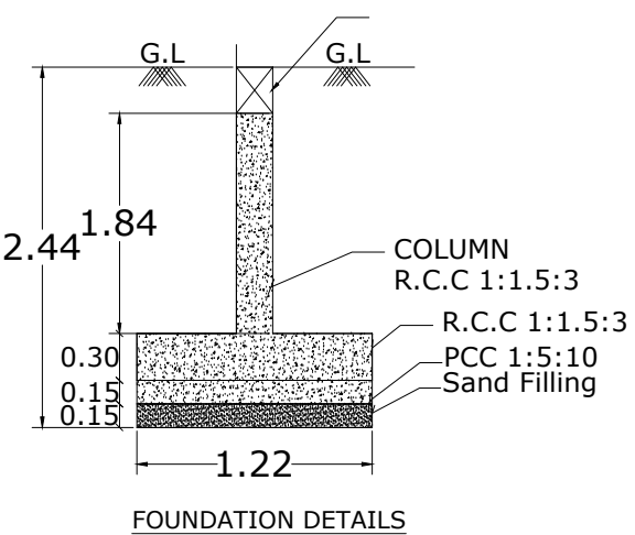
FOUNDATION DETAILS
