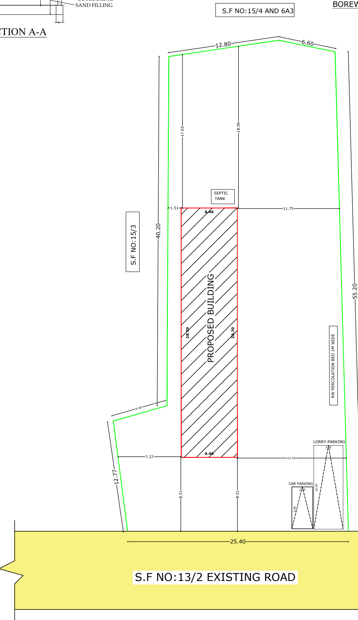
SITE PLAN
