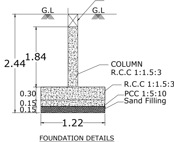
FOUNDATION DETAILS
