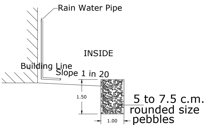
RAINWATER HARVESTING
