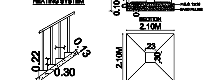
STAIRCASE DETAIL
