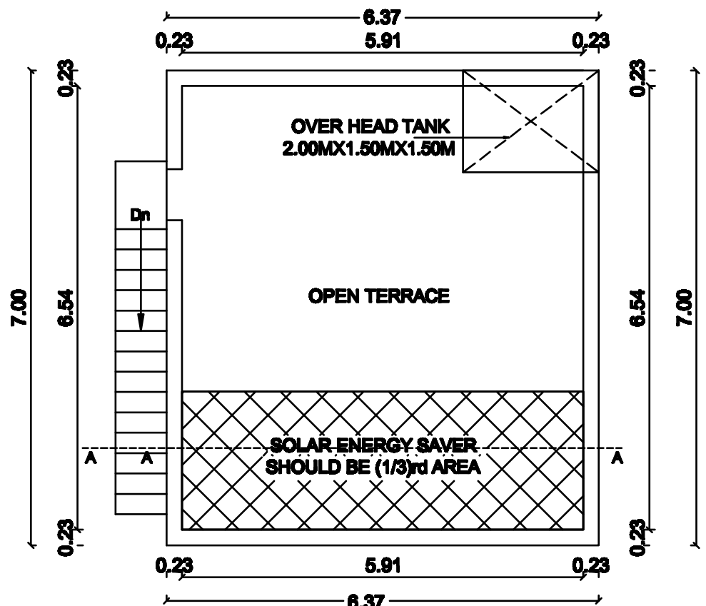
TERRACE FLOOR PLAN [PROPOSED]
