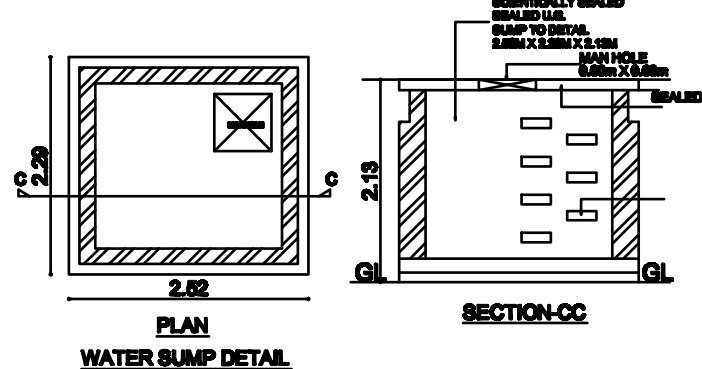
PLAN WATER SUMP DETAIL
