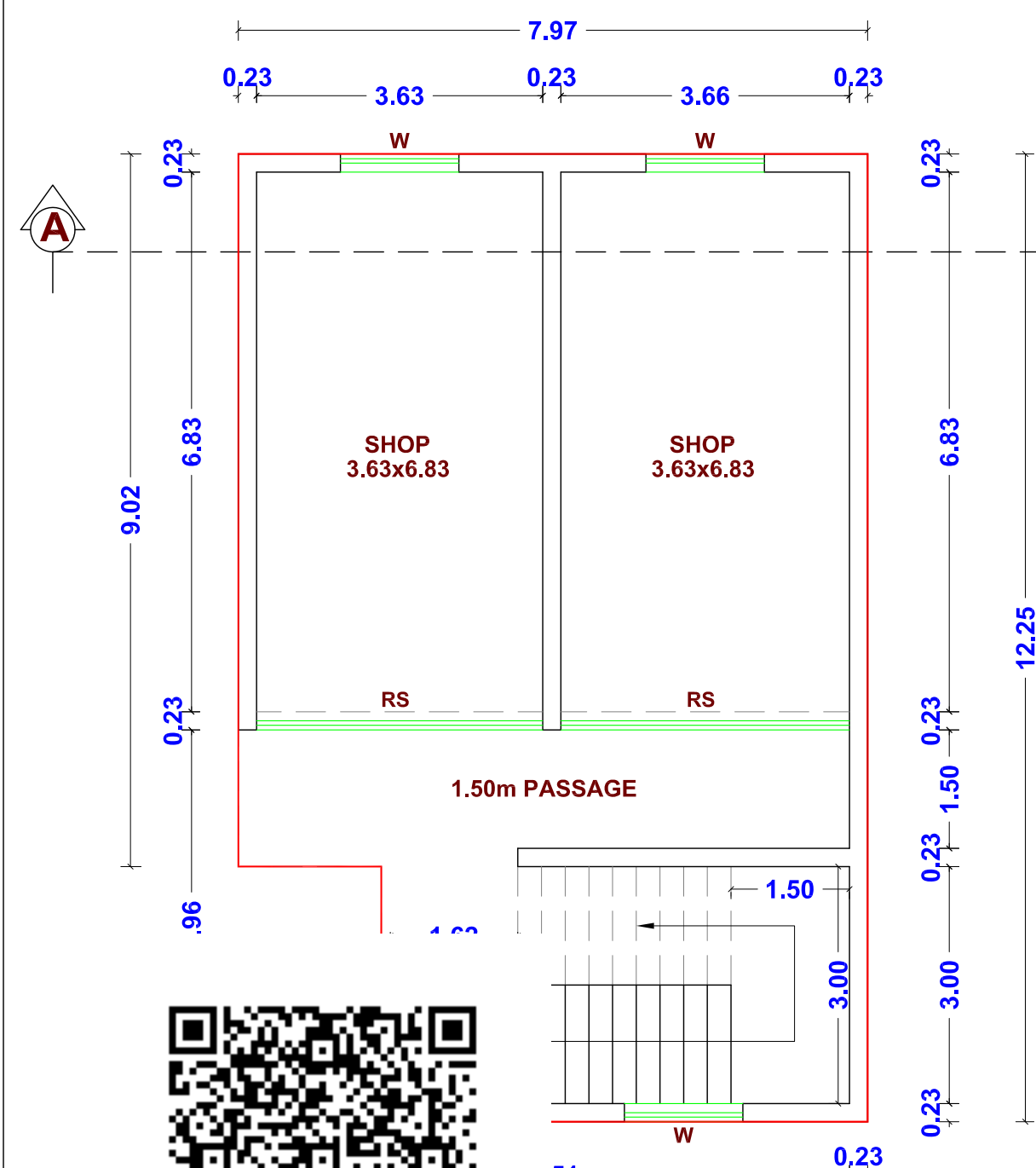
FLOOR PLAN
