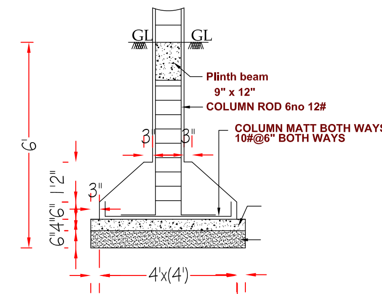
SECTION
