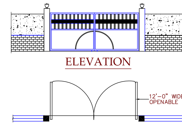
PLAN COMPOUND WALL DETAIL
