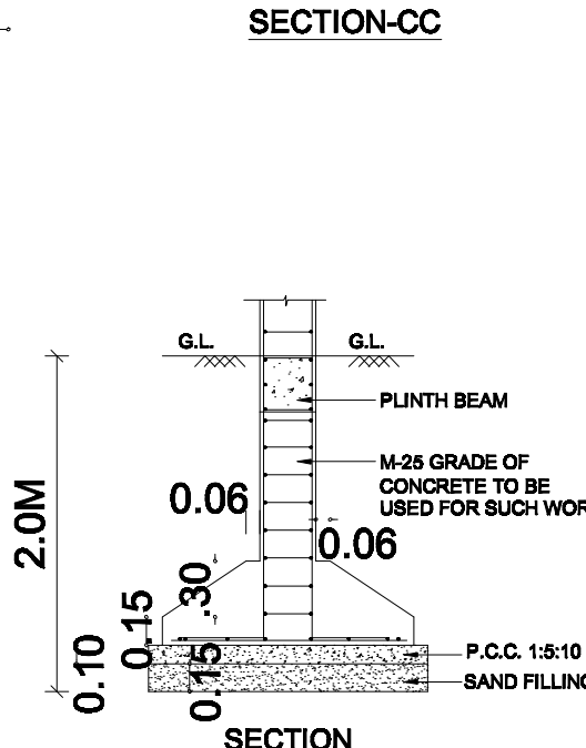
SECTION-CC
