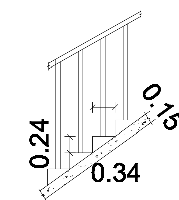
STAIRCASE DETAIL
