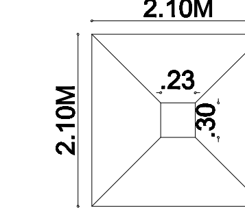
COLUMN PLAN SIZE: 0.23X0.30 TYPICAL FOUNDATION DETAIL
