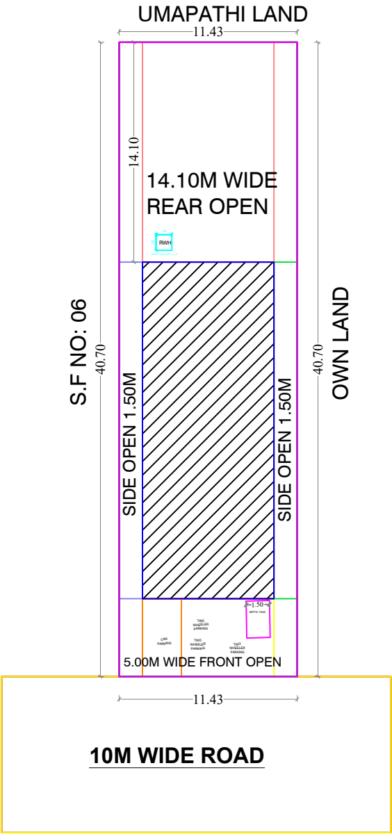
SITE PLAN
