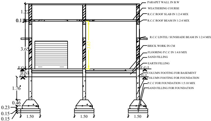
SECTION ON-AA
