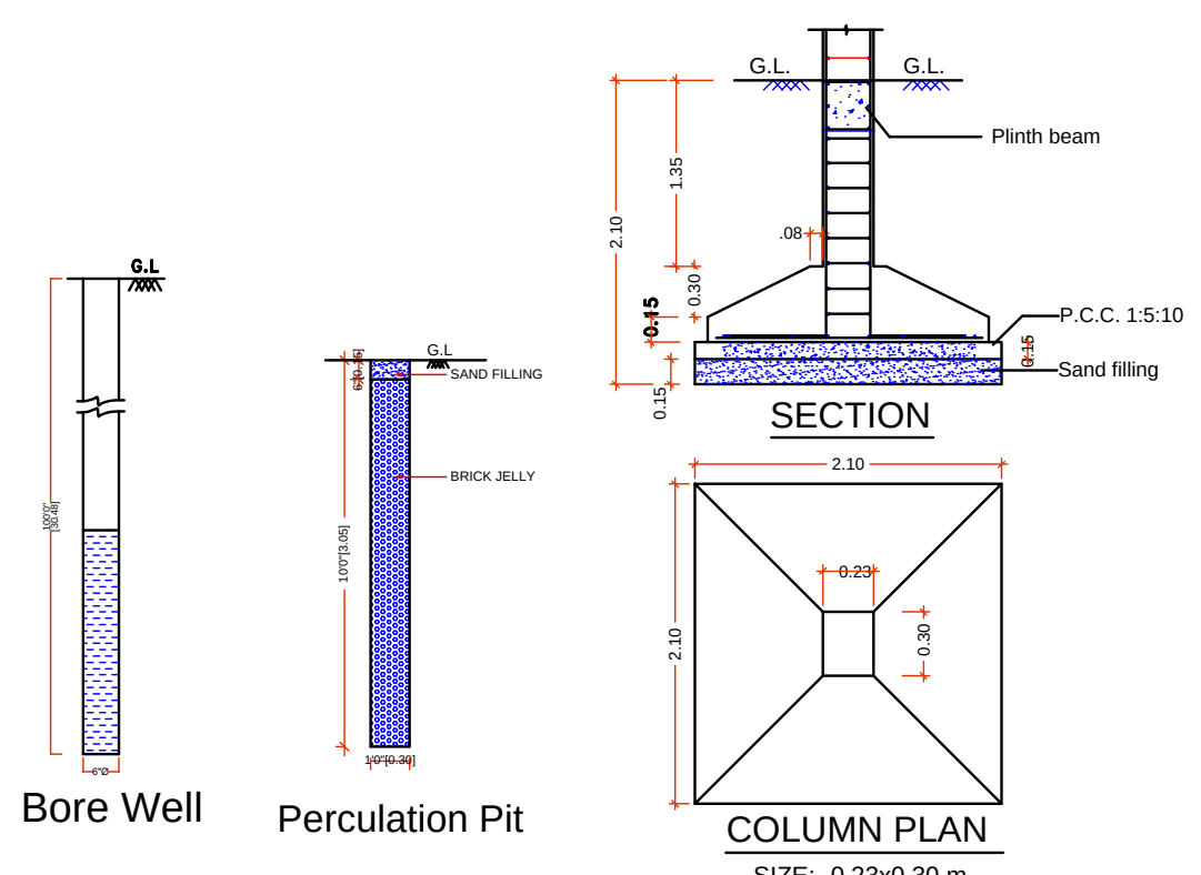
TYPICAL FOUNDATION DETAIL
