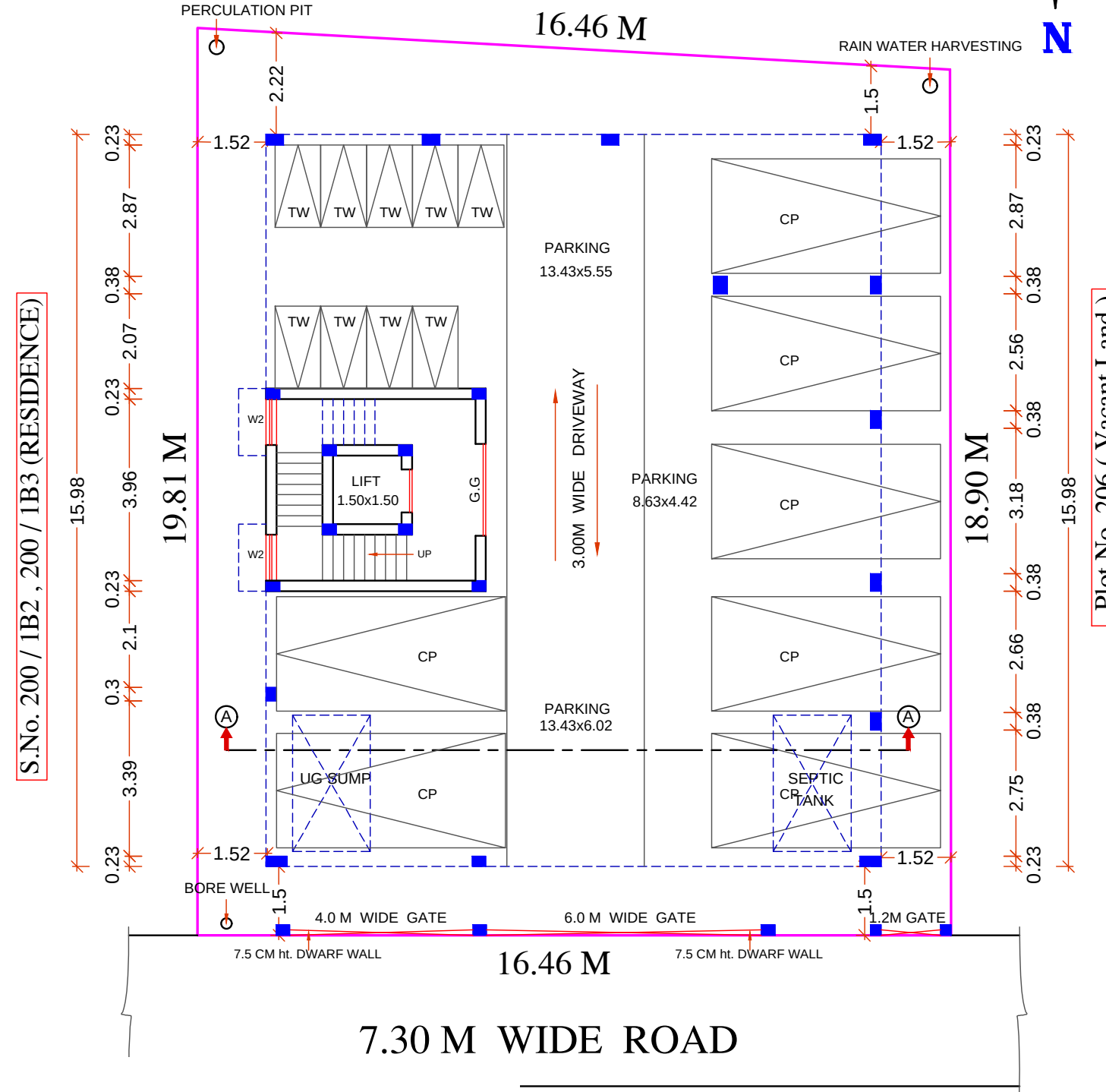
ILT FLOOR PLAN
