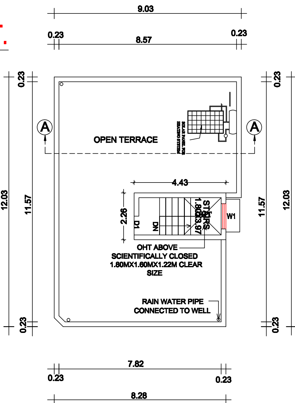
PRO.TERRACE FLOOR PLAN
