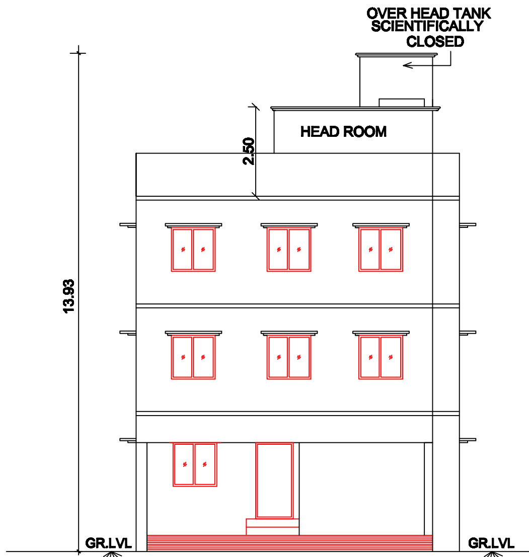
FRONT ELEVATION
