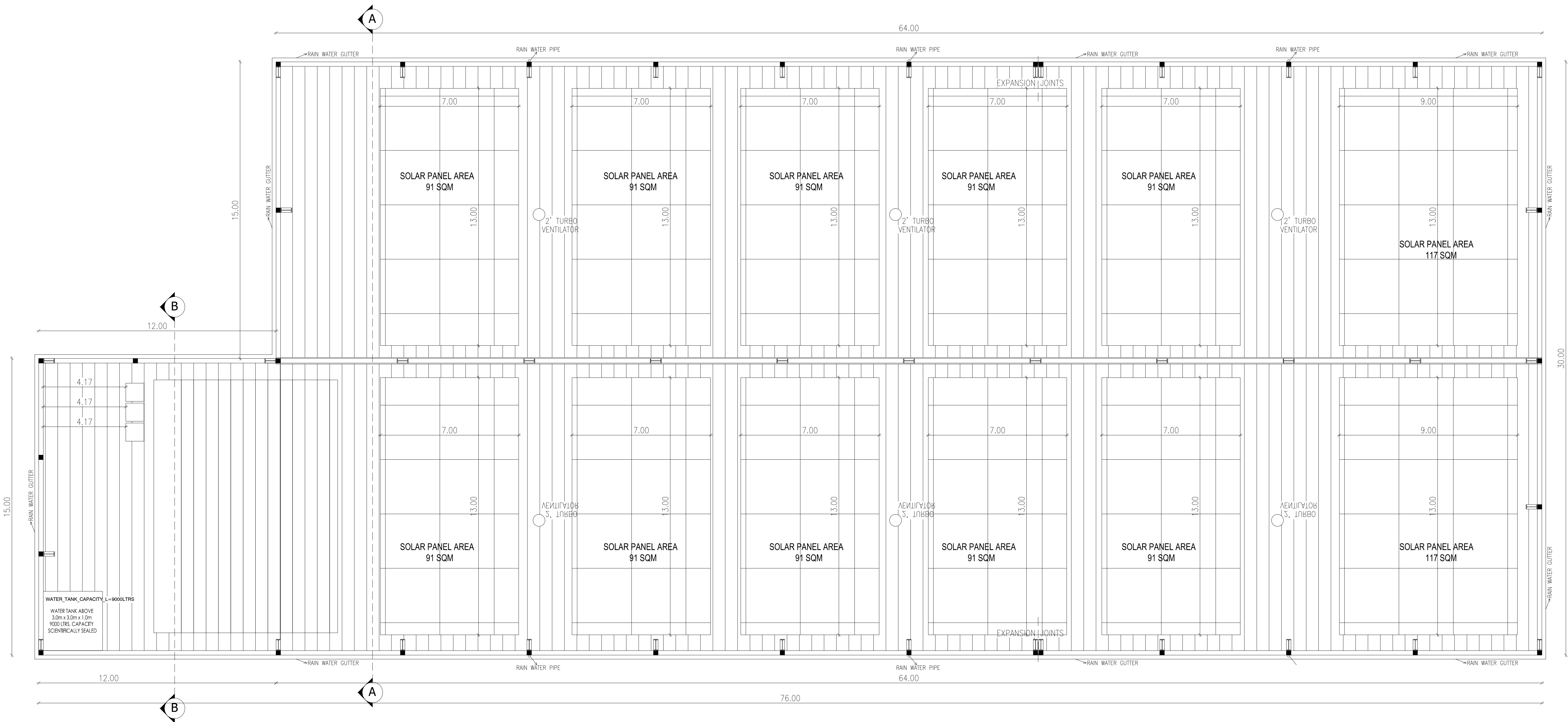
ROOF PLAN
