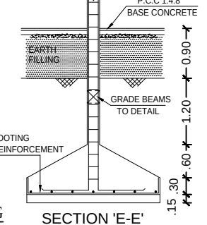
SECTION 'E-E'
