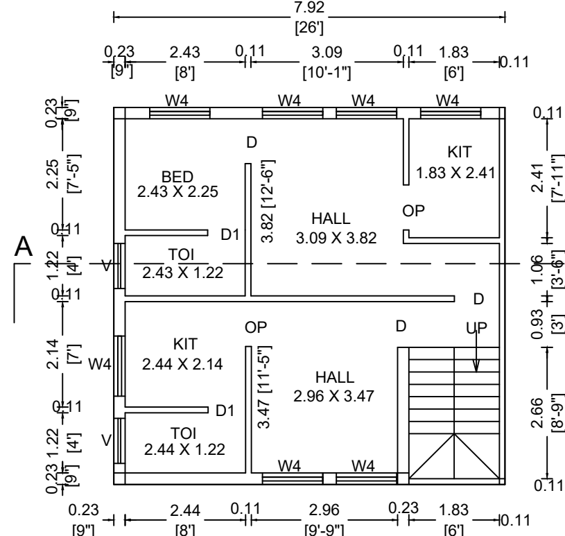
SECOND FLOOR PLAN (PROPOSED)
