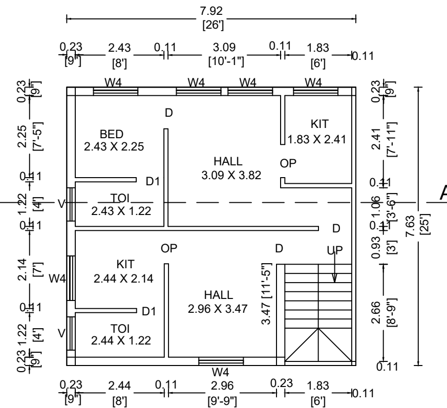
FIRST FLOOR PLAN (PROPOSED)
