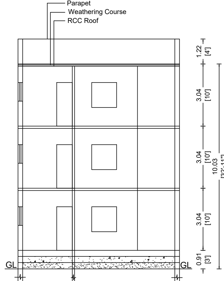
SECTION ON AA (PROPOSED)
