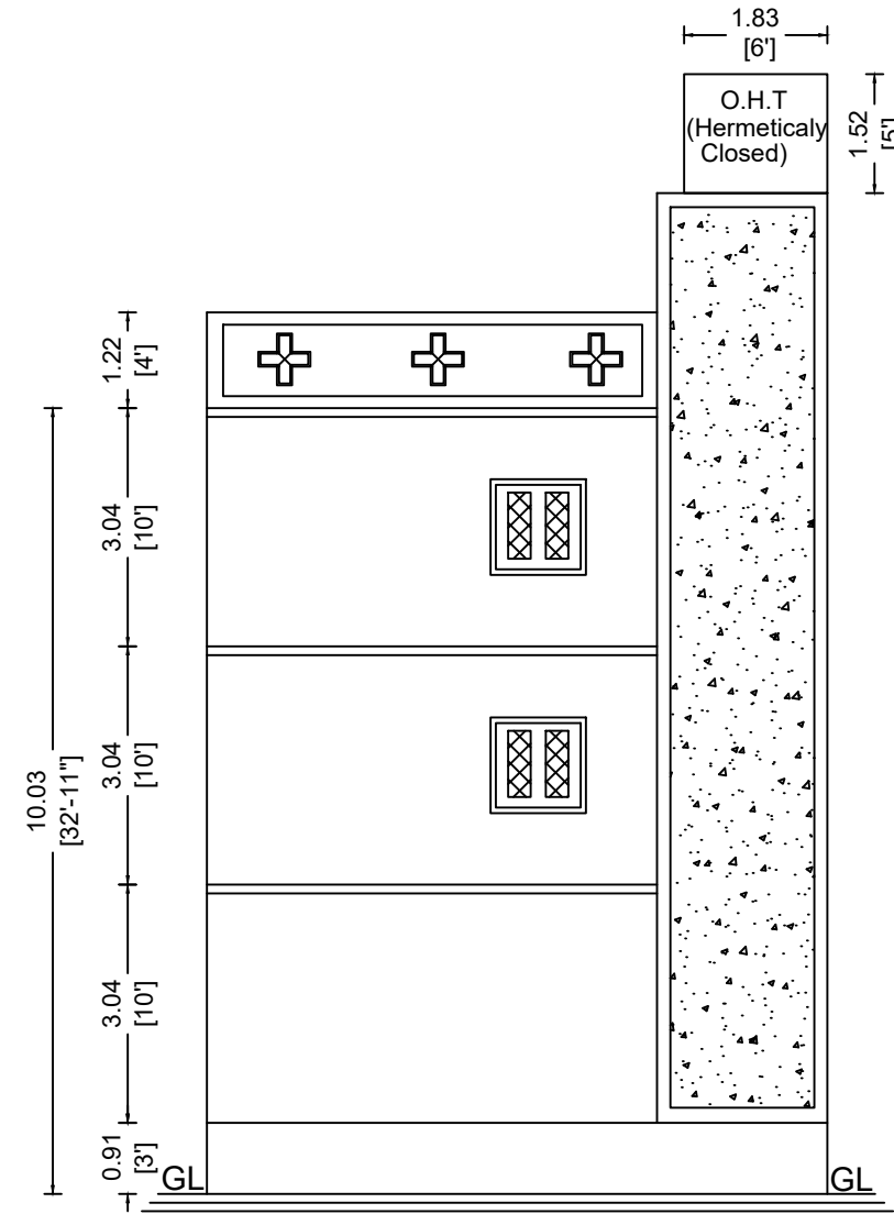
FRONT ELEVATION (PROPOSED)
