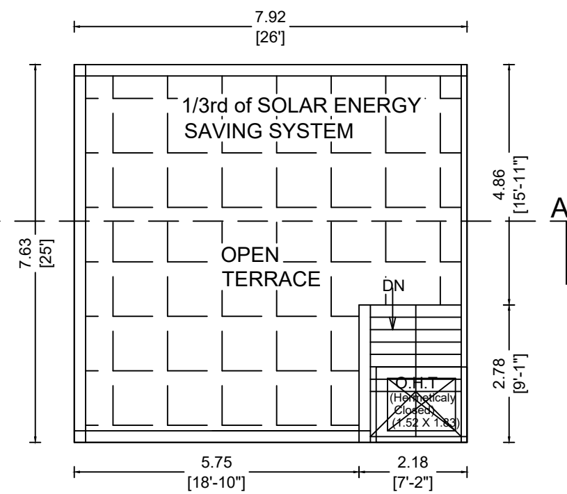
TERRACE FLOOR PLAN (PROPOSED)
