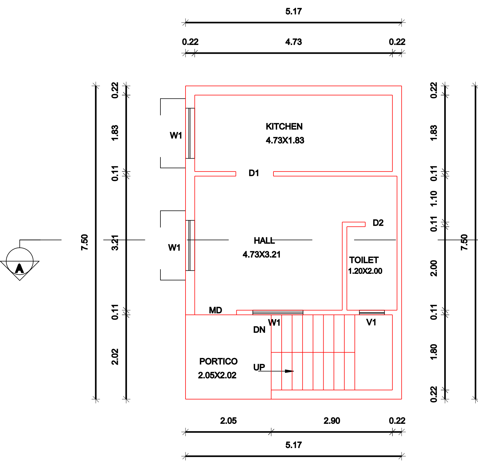
GROUND FLOOR PLAN FLOOR - 00 (PROPOSED)
