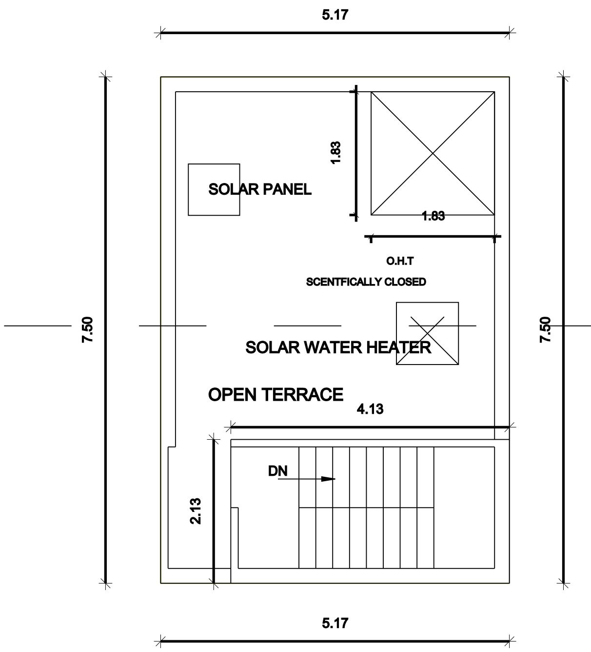
TERRACE FLOOR PLAN TERRACE (PROPOSED)
