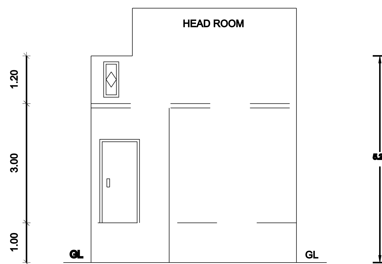
ELEVATION (PROPOSED)
