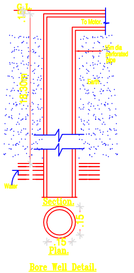
Bore Well Detail
