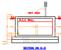
SECTION ON D-D
