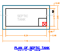
PLAN OF SEPTIC TANK SCALE 1"=2'-0"
