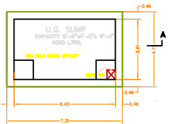
SUMP DETAIL SCALE 1"=2'-0"
