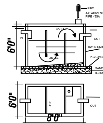
SEPTIC TANK
