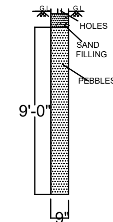
RAIN WATER PERCOLATION PIT
