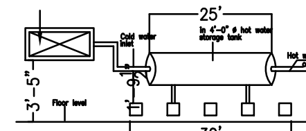
SOLAR HOT WATER SYSTEM(SWHS) DETAIL
