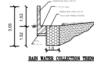
RAIN WATER COLLECTION TRENCH
