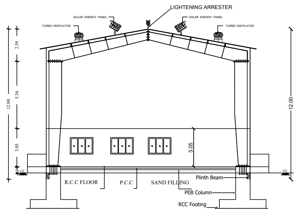
SECTION IN A-A
