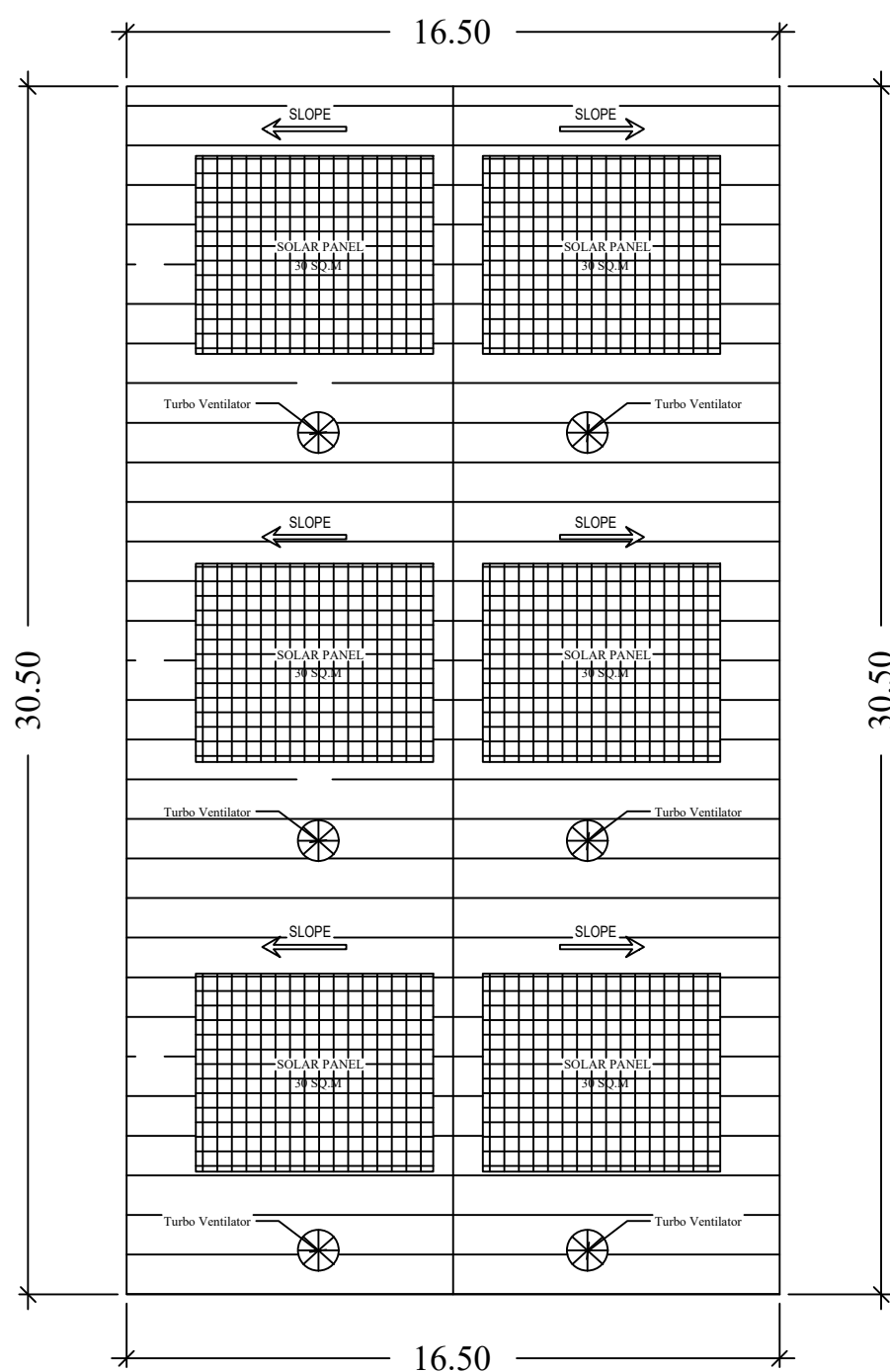
ROOF PLAN
