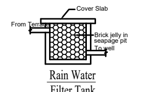
RAIN WATER Filter Tank
