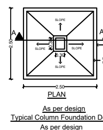
Typical Column Foundation Detail As per design
