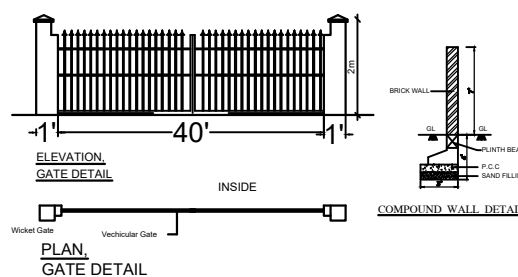
PLAN, GATE DETAIL
