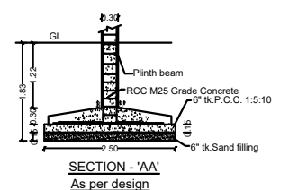
SECTION 'AA' As per design
