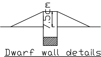
Dwarf wall details
