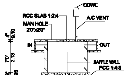
SECTION OF S.TANK
