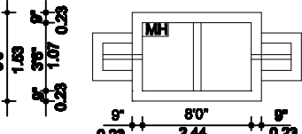
PLAN - SEPTIC TANK
