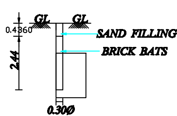
CROSS SECTION OF PERCOLATION PIT
