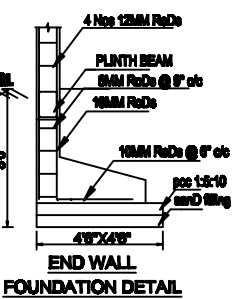
END WALL FOUNDATION DETAIL
