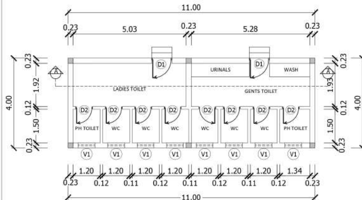
TOILET BLOCK - 3
