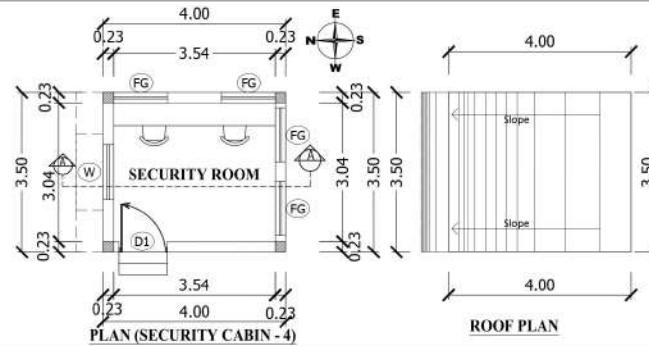
PLAN (SECURITY CABIN - 4)
