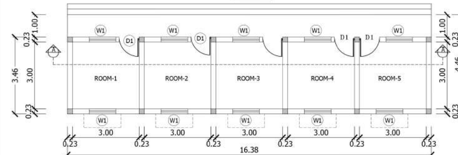
LABOUR ROOM - 2
