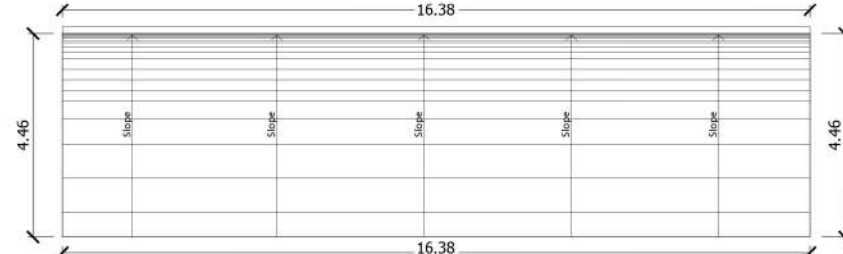
ROOF PLAN
