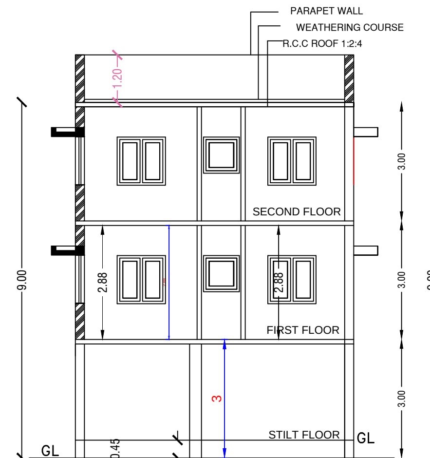
SECTION ON AB (PROPOSED)
