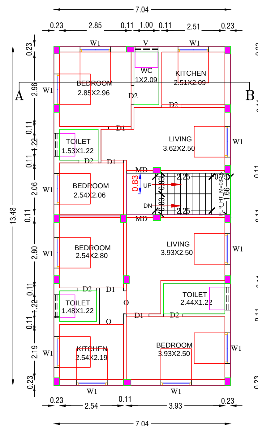
SECOND FLOOR PLAN PROPOSED
