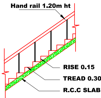
STAIRCASE DETAIL
