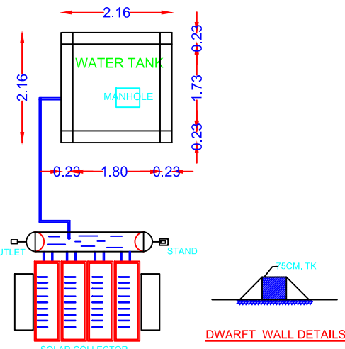
PLAN OF OHT SOLAR WATER HEATING SYSTEM
