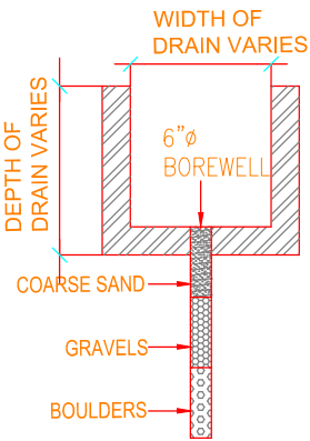
BOREWELL DETAIL (SCALE= 1:50)
