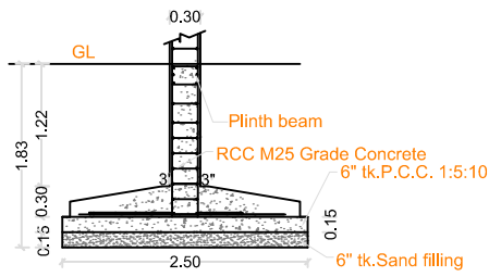
SECTION - 'AA' As per design
