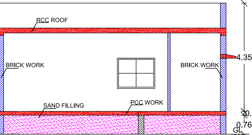
SECTION ON-AA
