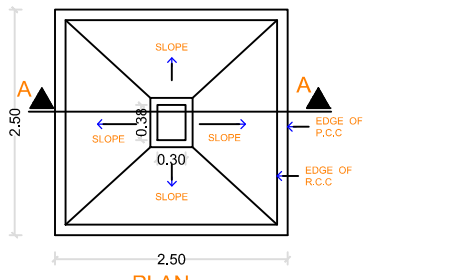
As per design Typical Column Foundation Detail As per design
