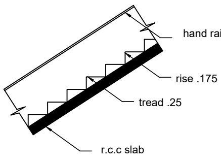
STAIR
