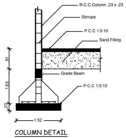
COLUMN DETAIL
