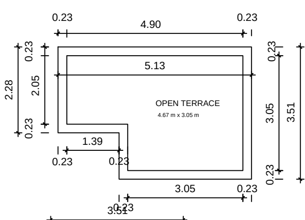
TERMINAL FLOOR PLAN (TO BE DEMOLISHED)
