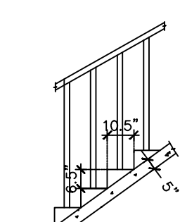
STAIRCASE SECTION
