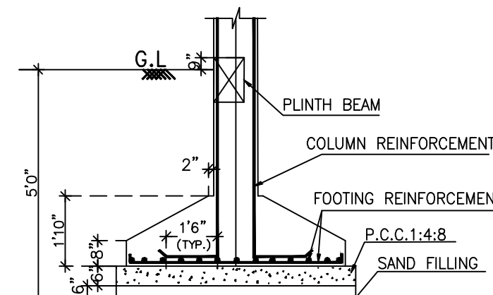
SECTION X-X
