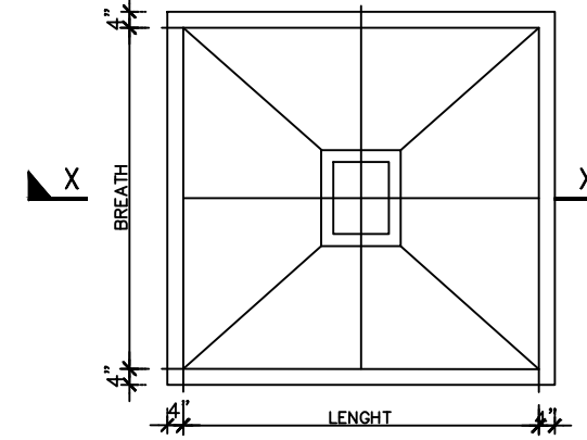
FOOTING DETAIL
