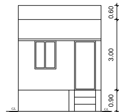
ELEVATION (TO BE DEMOLISHED)
