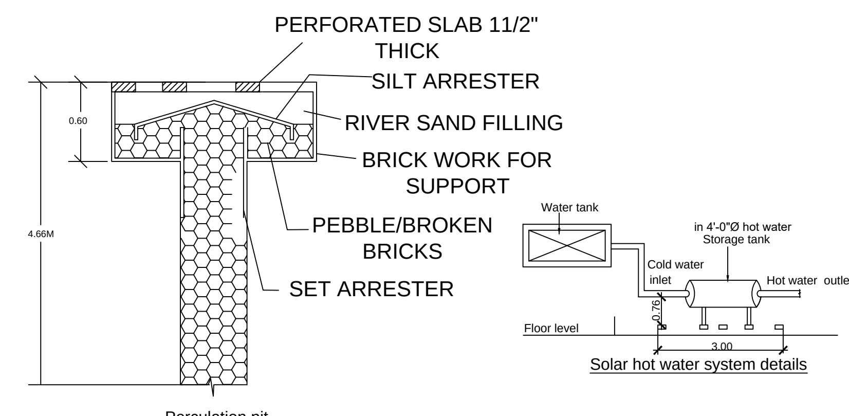
Percolation p
