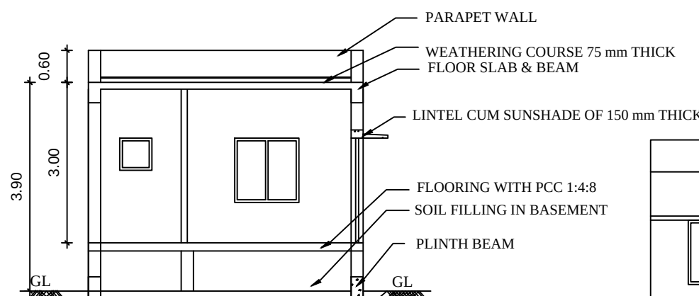
SECTION A-A (TO BE DEMOLISHED)
