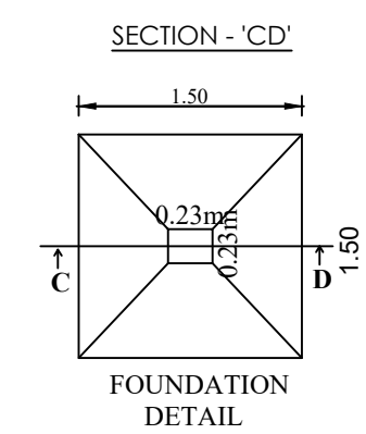
SECTION - 'CD'
