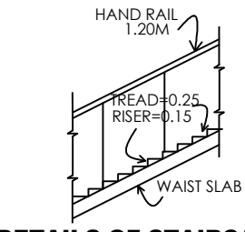
DETAILS OF STAIRCASE (Not to Scale)
