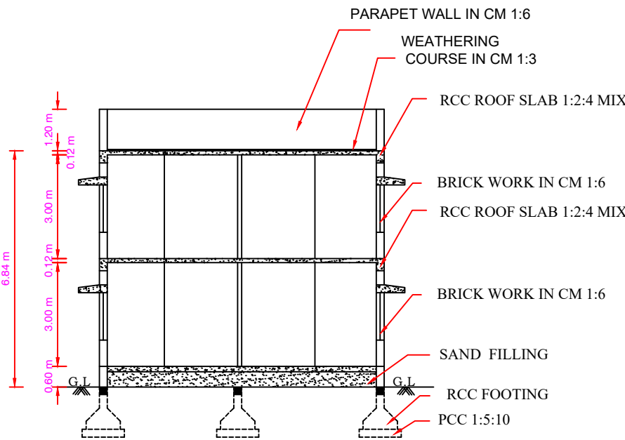
SECTION-AB
