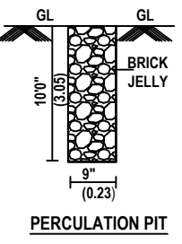
PERCOLATION PIT
