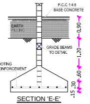
DETAILS OF COLUMN FOOTING
