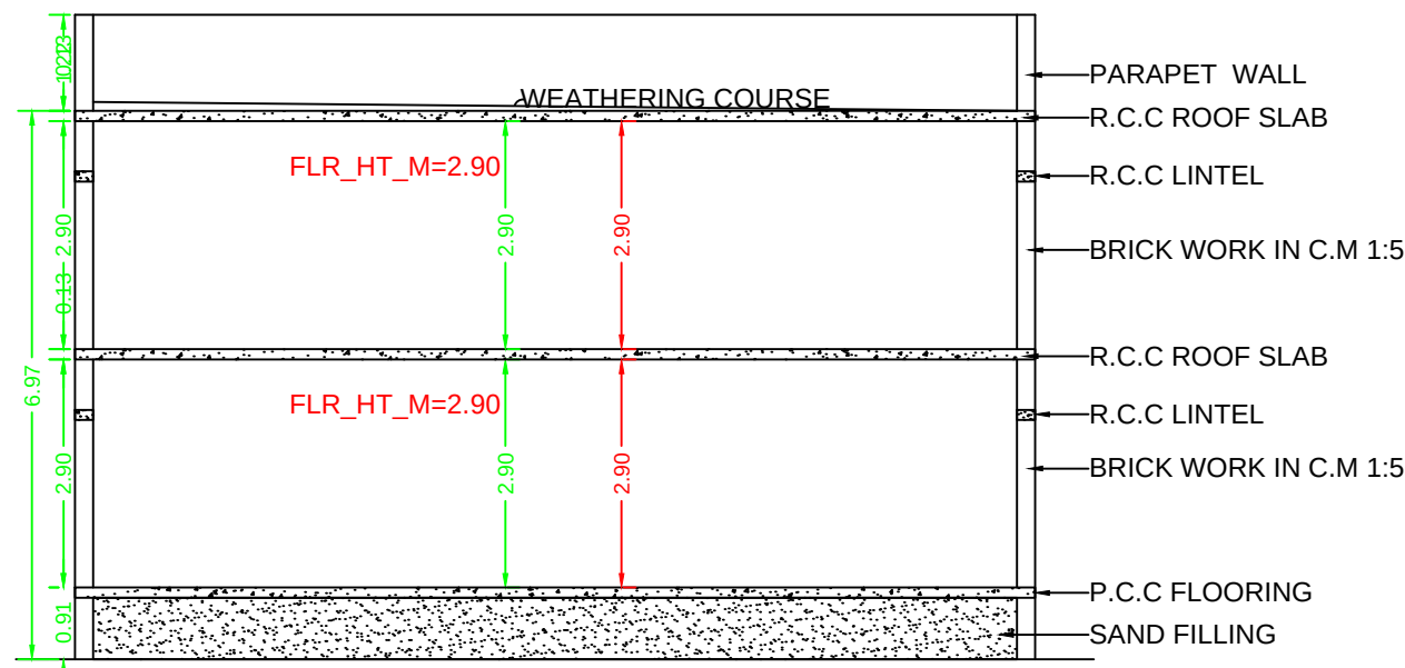
SECTION
