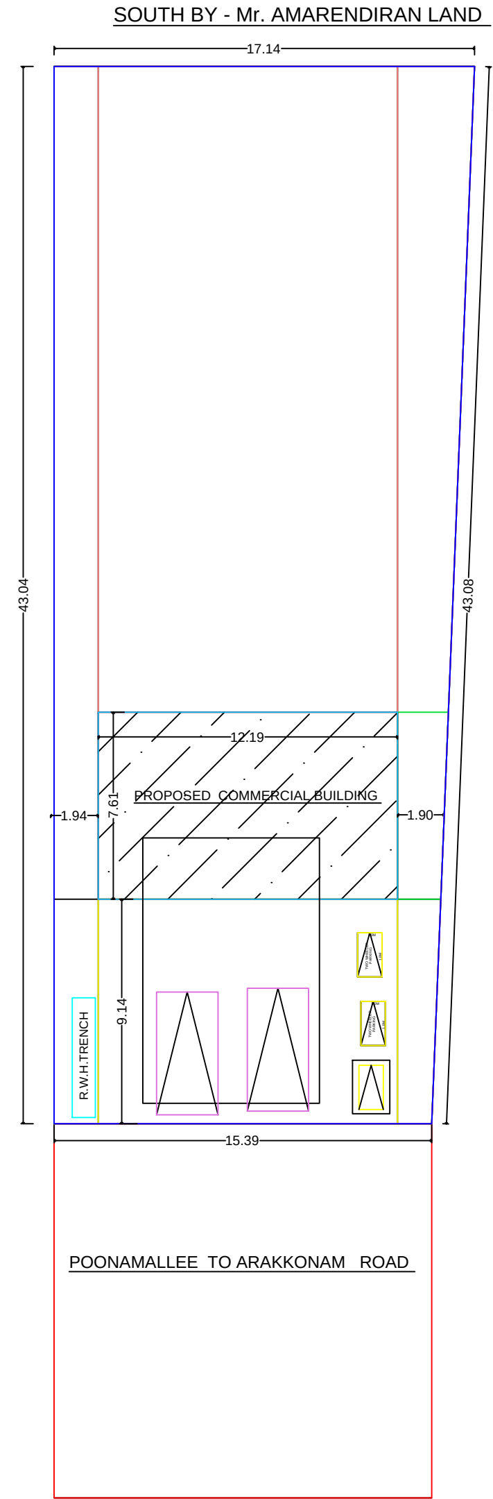
SITE PLAN
