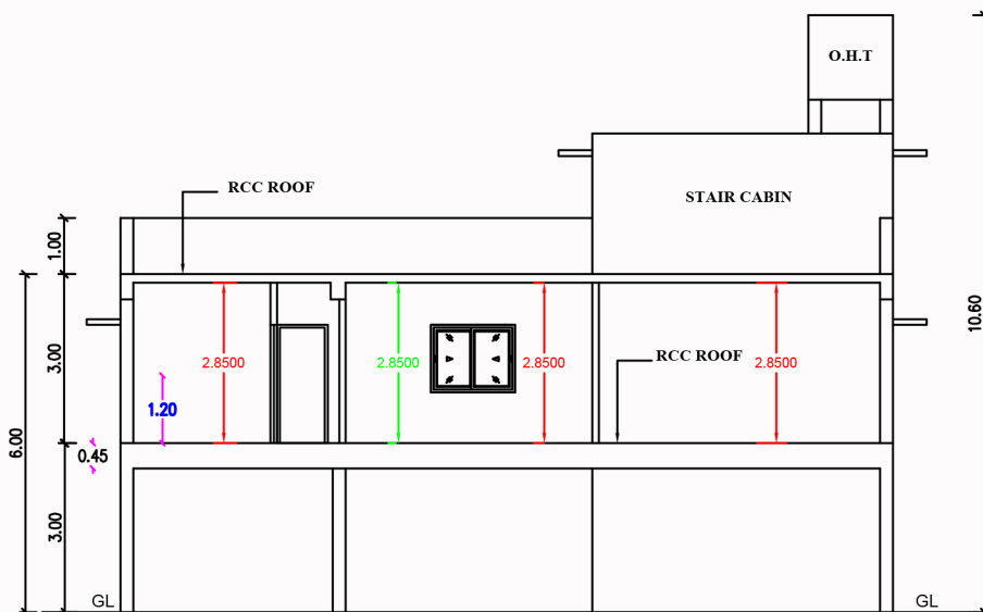
SECTION ON A-A (PROPOSED)
