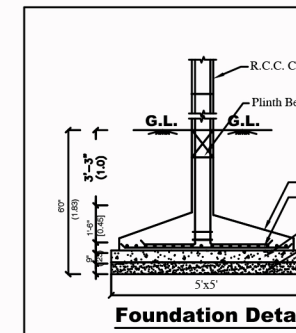
Foundation Det
