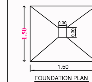
FOUNDATION PLAN
