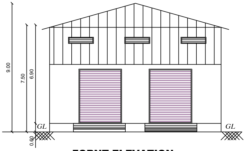
FORNT ELEVATION
