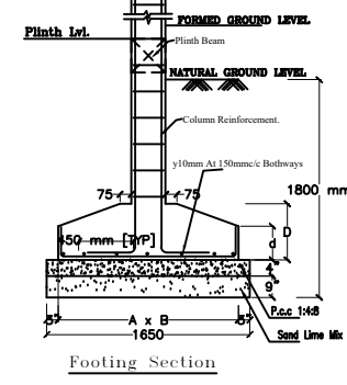
Footings Section
