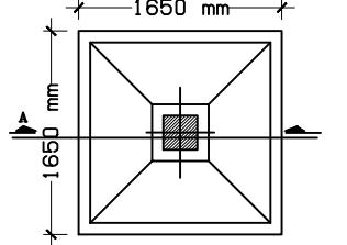
Footings Plan
