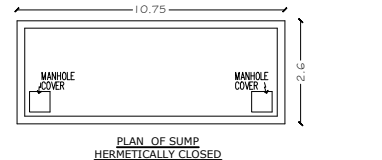
PLAN OF SUMP
