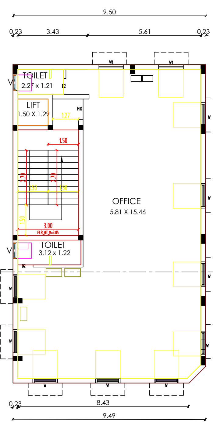
FIRST FLOOR PLAN (PROPOSED - COMMERCIAL)
