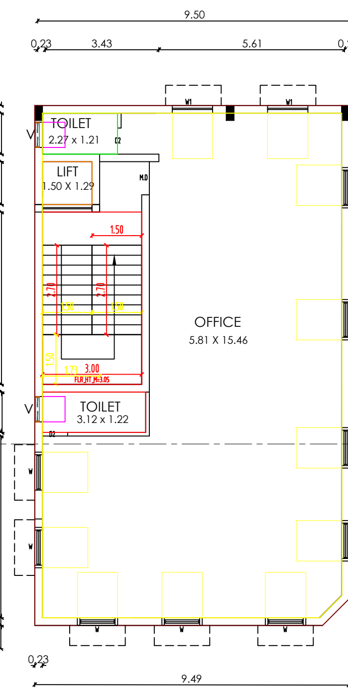
SECOND FLOOR PLAN (PROPOSED - COMMERCIAL)
