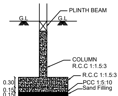
Foundation Details
