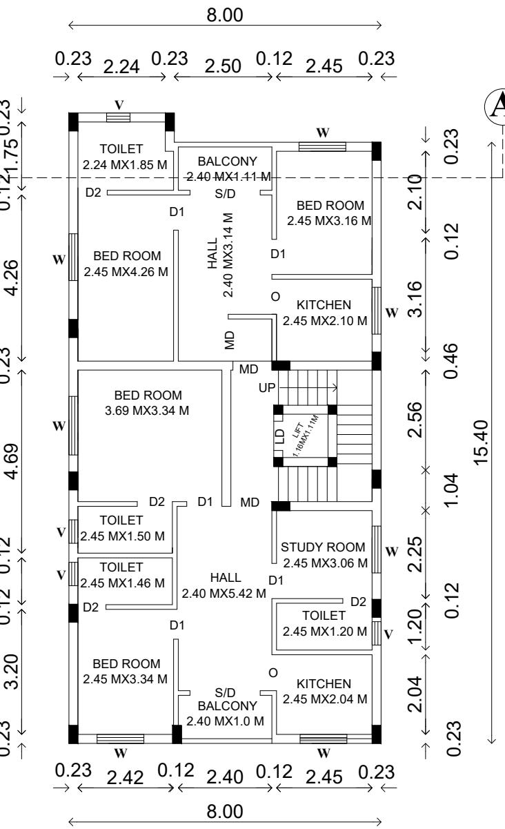
THIRD FLOOR PLAN PROPOSED
