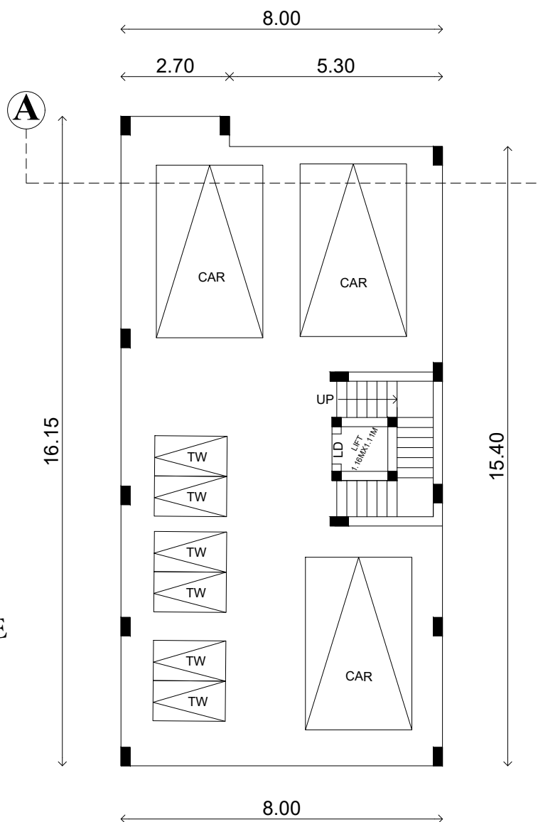
STILT FLOOR PLAN PROPOSED
