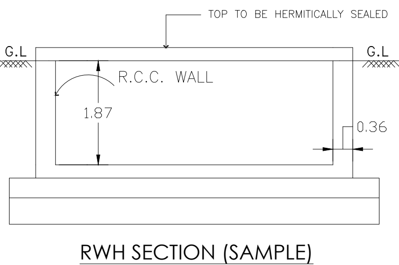
RWTH SECTION (SAMPLE)
