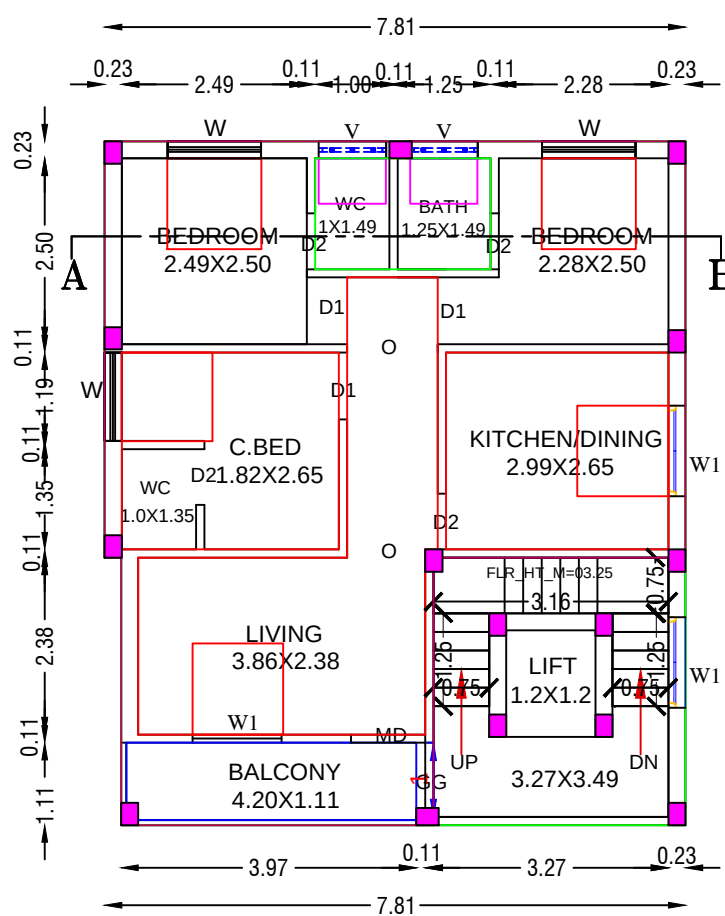
THIRD FLOOR PLAN (PROPOSED)
