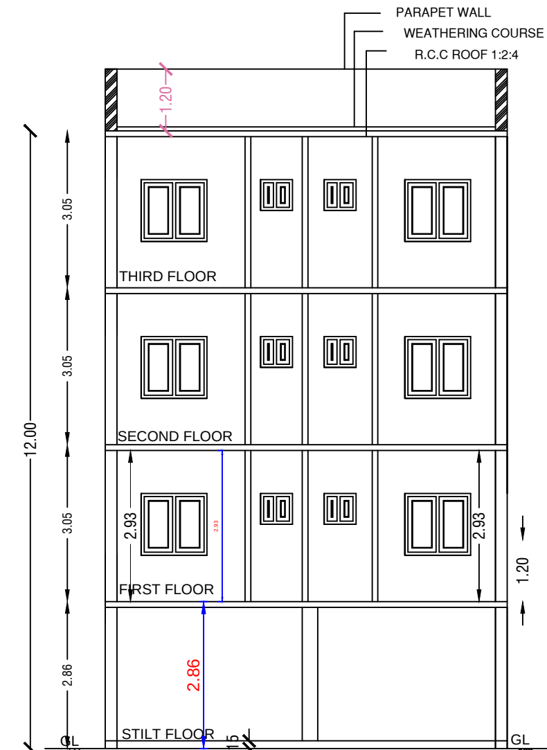
SECTION ON AB (PROPOSED)
