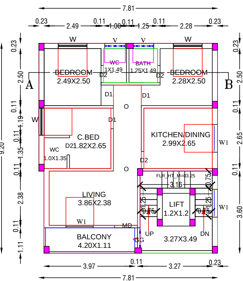
SECOND FLOOR PLAN (PROPOSED)
