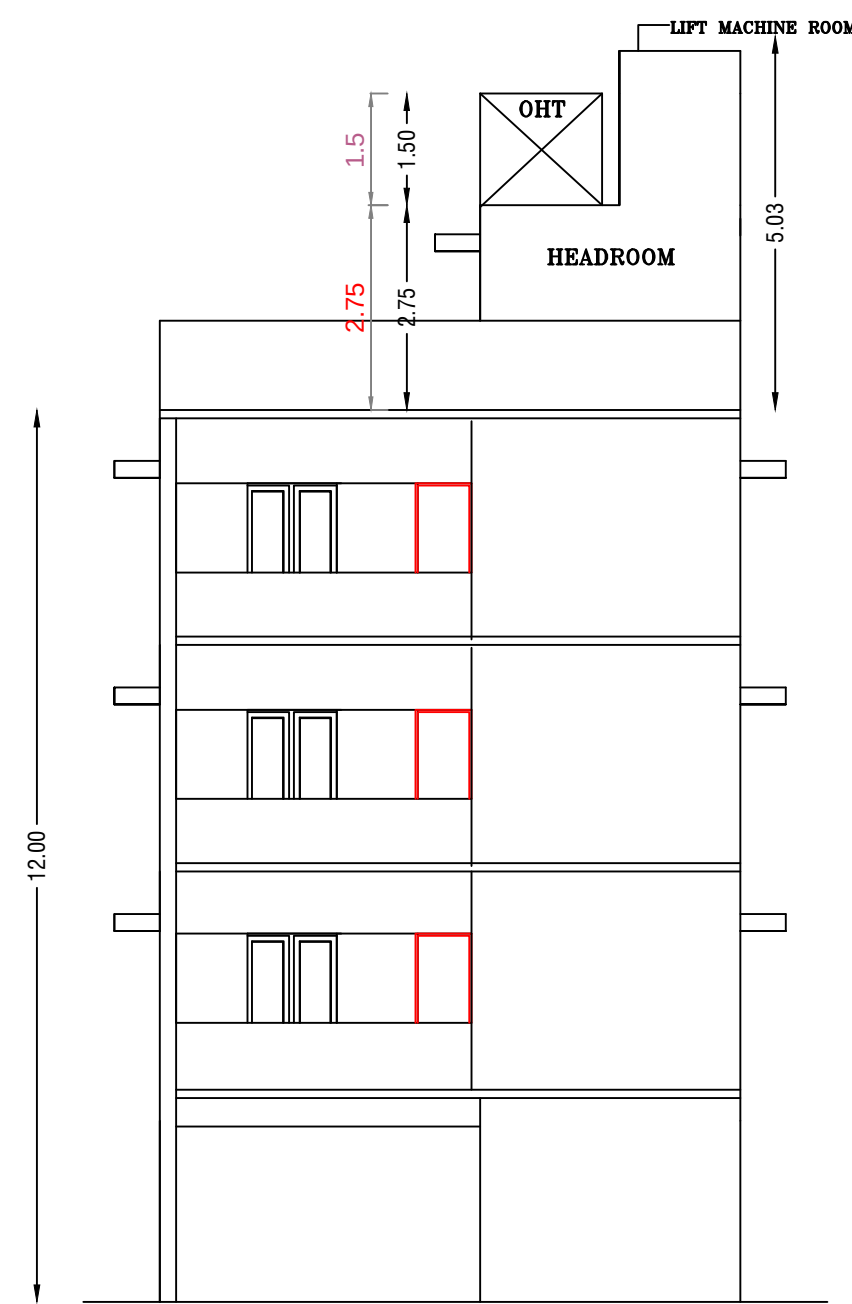
FRONT ELEVATION (PROPOSED)
