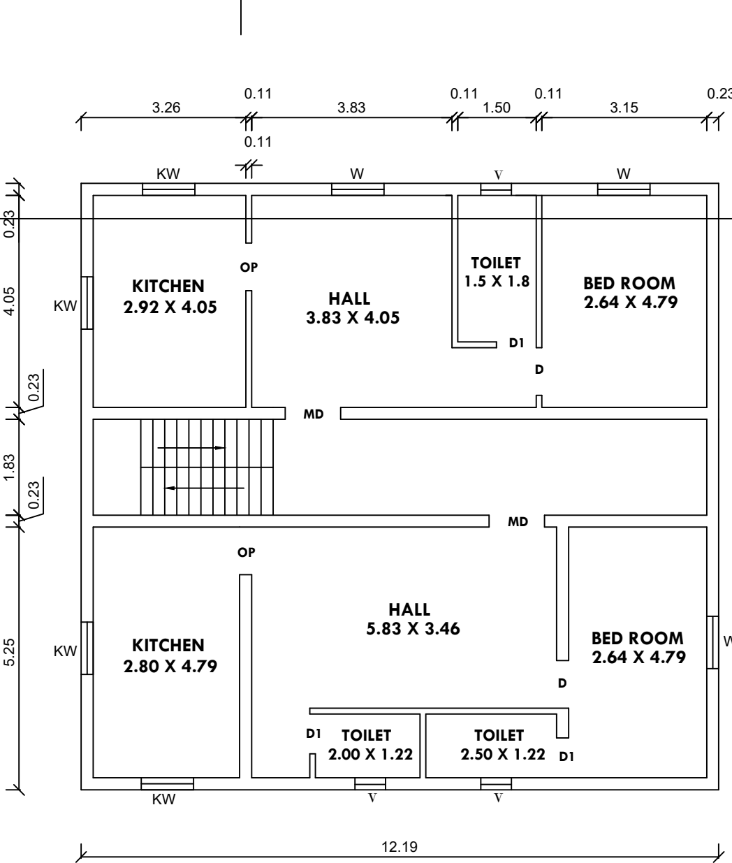
PRO.SECOND FLOOR PLAN
